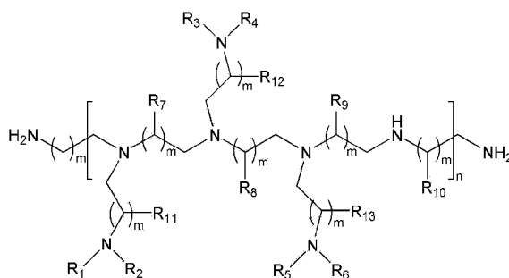
[Chemical Formula 1]
