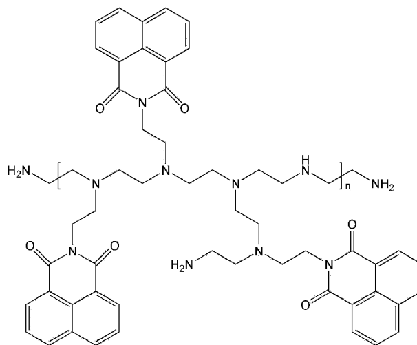
[Chemical Formula 2]
