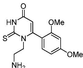
1-(2-aminoethyl)-6-(2,4-dimethoxyphenyl)-2-thioxo-2,3-dihydropyrimidin-4(1H)-one hydrochloride
