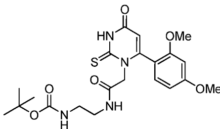
tert-Butyl (2-(2-(6-(2,4-dimethoxyphenyl)-4-oxo-2-thioxo-3,4-dihydropyrimidin-1(2H)-yl)acetamido)ethyl)carbamate
