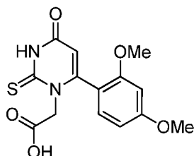
2-(6-(2,4-dimethoxyphenyl)-4-oxo-2-thioxo-3,4-dihydropyrimidin-1(2H)-yl)acetic acid
