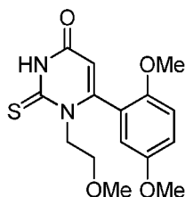
6-(2,5-dimethoxyphenyl)-1-(2-methoxyethyl)-2-thioxo-2,3-dihydropyrimidin-4(1H)-one
