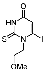
6-Iodo-1-(2-methoxyethyl)-2-thioxo-2,3-dihydropyrimidin-4(1H)-one
