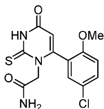
2-(6-(5-Chloro-2-methoxyphenyl)-4-oxo-2-thioxo-3,4-dihydropyrimidin-1(2H)-yl) acetamide
