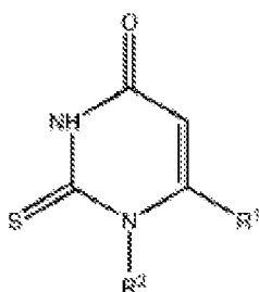
Formula I
