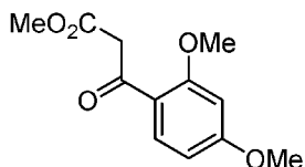
Methyl 3-(2,4-dimethoxyphenyl)-3-oxopropanoate
