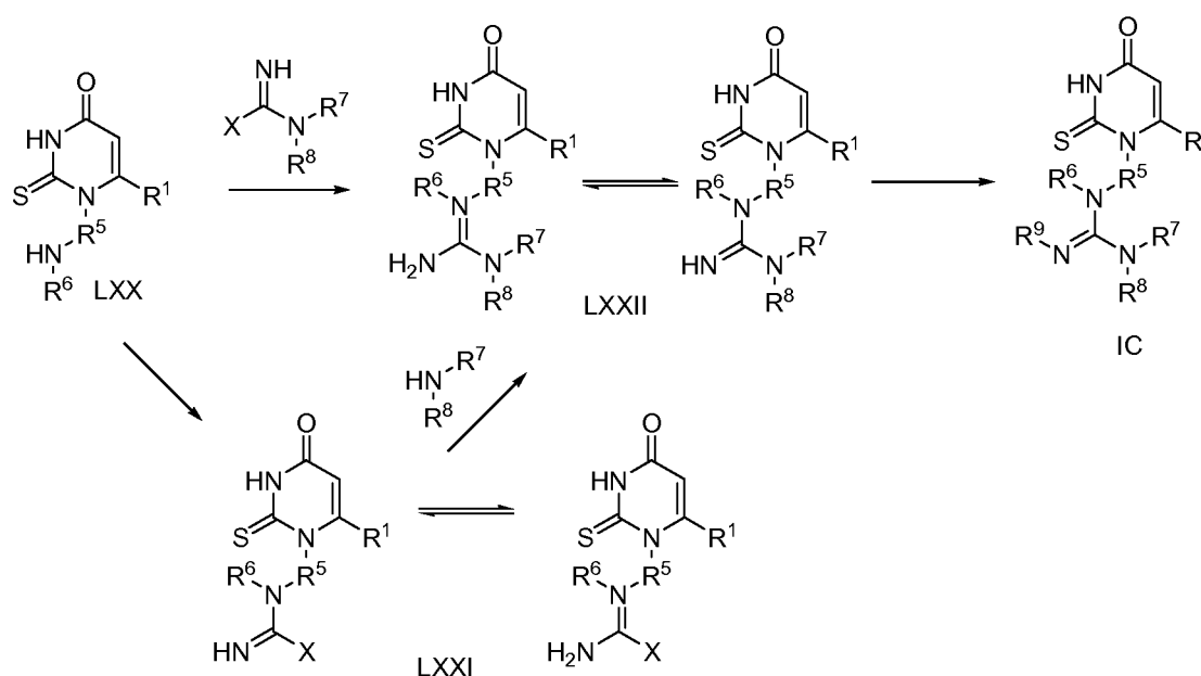
SCHEME IV
