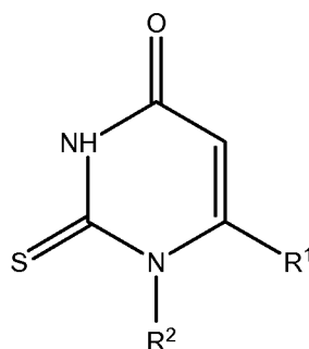
Formula IA
