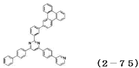
[Chemical Formula 152]
