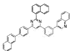
[Chemical Formula 104]
