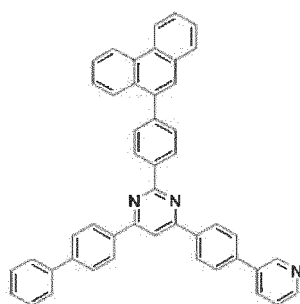
[Chemical Formula 146]
