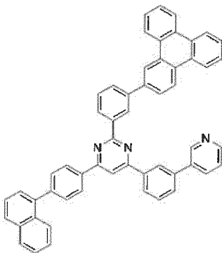
[Chemical Formula 195]
