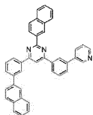
[Chemical Formula 117]
