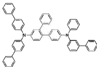
[Chemical Formula 69]
