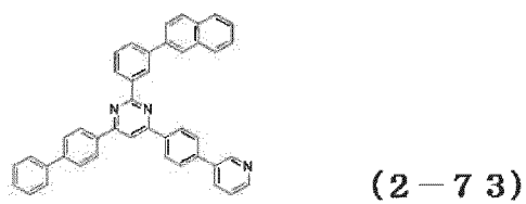
[Chemical Formula 150]
