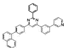
[Chemical Formula 91]
