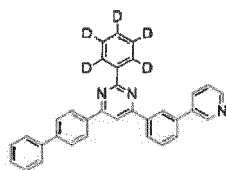
[Chemical Formula 79]
