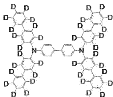
[Chemical Formula 225]
