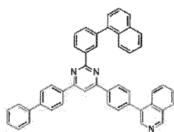
[Chemical Formula 180]
