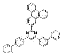
[Chemical Formula 82]
