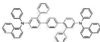
[Chemical Formula 44]
