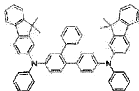
[Chemical Formula 66]
