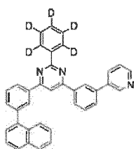
[Chemical Formula 100]
