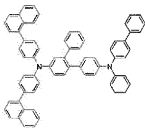
[Chemical Formula 62]
