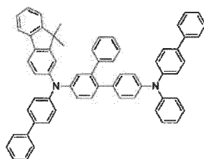
[Chemical Formula 64]
