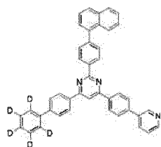
[Chemical Formula 185]
