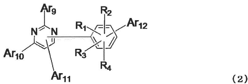
[Chemical Formula 3]
