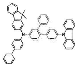
[Chemical Formula 66]
