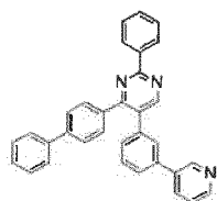
[Chemical Formula 126]
