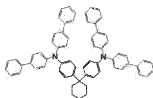
[Chemical Formula 209]
