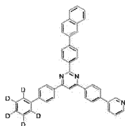
[Chemical Formula 185]
