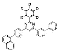
[Chemical Formula 91]
