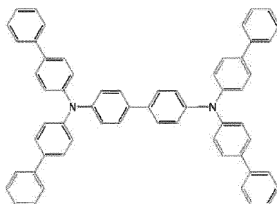
[Chemical Formula 253]
