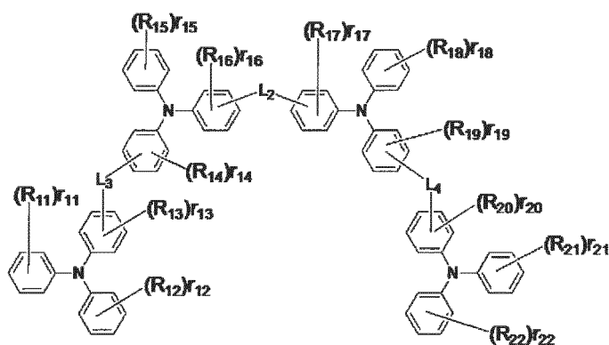
[Chemical Formula 27]
