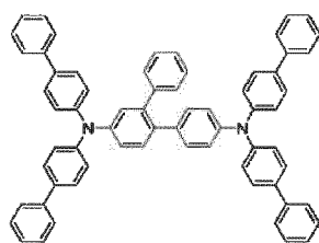
[Chemical Formula 59]
