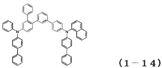
[Chemical Formula 48]
