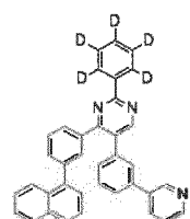
[Chemical Formula 137]
