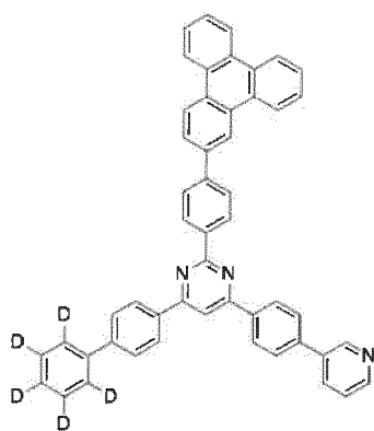
[Chemical Formula 187]
