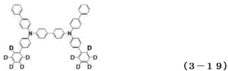
[Chemical Formula 222]
