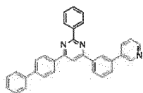
[Chemical Formula 77]
