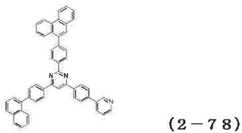
[Chemical Formula 155]
