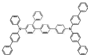
[Chemical Formula 38]
