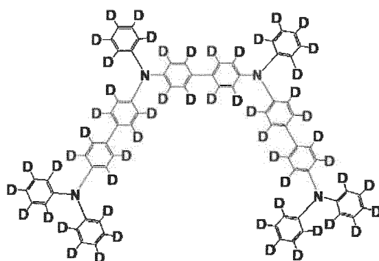
[Chemical Formula 241]
