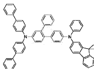
[Chemical Formula 74]
