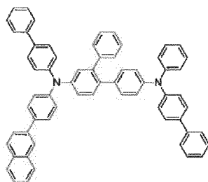
[Chemical Formula 60]
