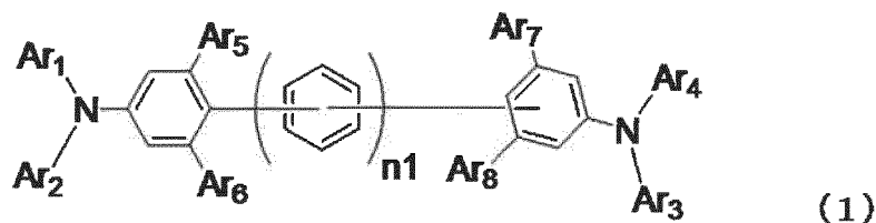
[Chemical Formula 17]
