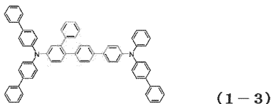
[Chemical Formula 36]
