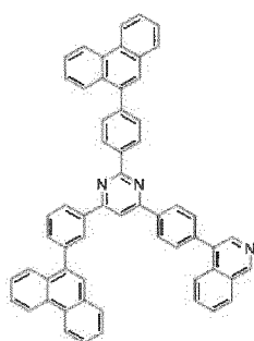
[Chemical Formula 170]
