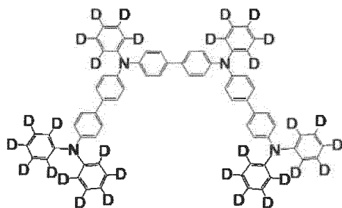
[Chemical Formula 240]
