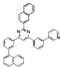
[Chemical Formula 99]
