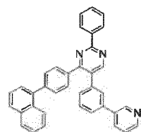
[Chemical Formula 132]
