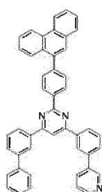
[Chemical Formula 191]
