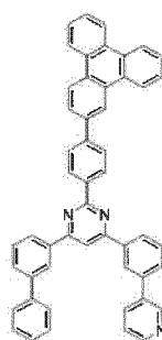
[Chemical Formula 191]
