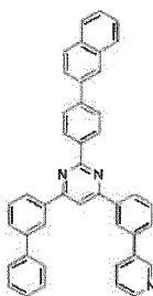
[Chemical Formula 189]
