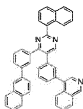
[Chemical Formula 136]
