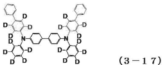
[Chemical Formula 219]
