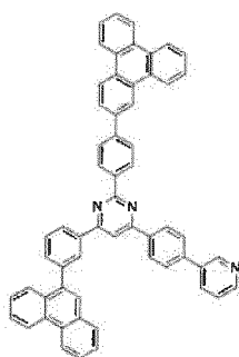
[Chemical Formula 171]
