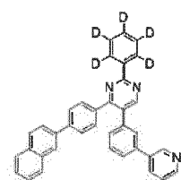
[Chemical Formula 134]
