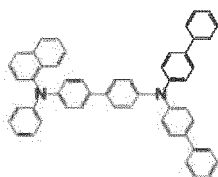
[Chemical Formula 216]
