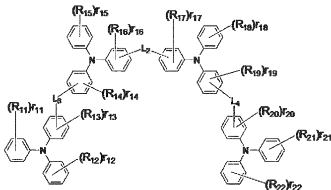
[Chemical Formula 10]
