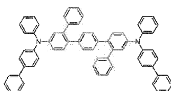
[Chemical Formula 259]
