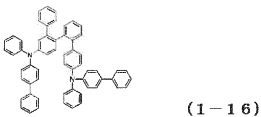
[Chemical Formula 50]
