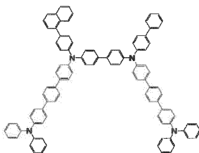
[Chemical Formula 231]
