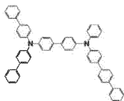
[Chemical Formula 206]
