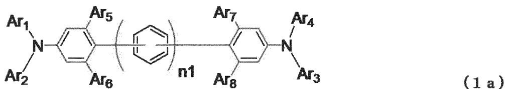
[Chemical Formula 18]
