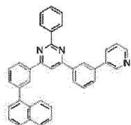
[Chemical Formula 96]
