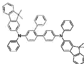
[Chemical Formula 71]
