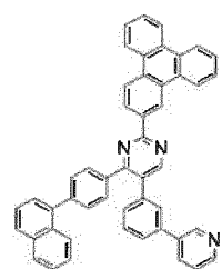
[Chemical Formula 133]
