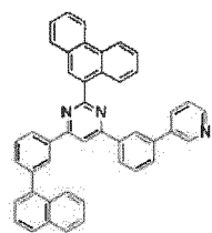
[Chemical Formula 101]
