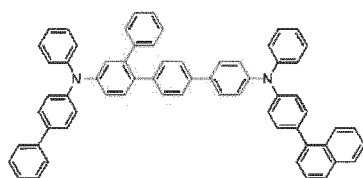
[Chemical Formula 40]
