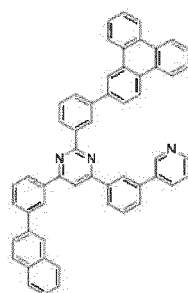
[Chemical Formula 198]
