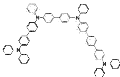
[Chemical Formula 230]
