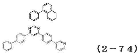
[Chemical Formula 151]
