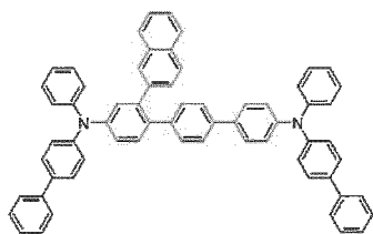
[Chemical Formula 41]
