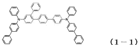
[Chemical Formula 35]
