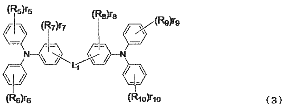
[Chemical Formula 21]
