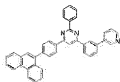
[Chemical Formula 121]
