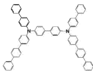
[Chemical Formula 205]
