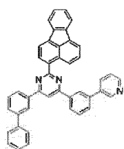
[Chemical Formula 90]
