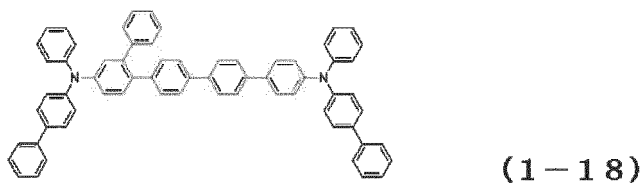
[Chemical Formula 51]
