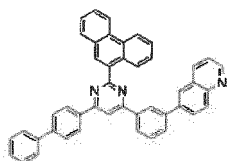
[Chemical Formula 82]
