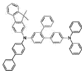
[Chemical Formula 68]
