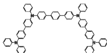
[Chemical Formula 227]
