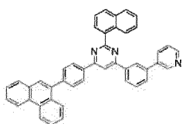
[Chemical Formula 123]
