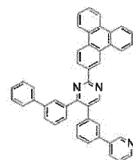
[Chemical Formula 132]
