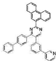
[Chemical Formula 127]
