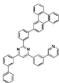
[Chemical Formula 196]
