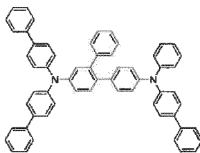
[Chemical Formula 57]
