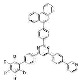
[Chemical Formula 186]
