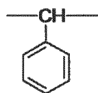
[Chemical Formula 25]
