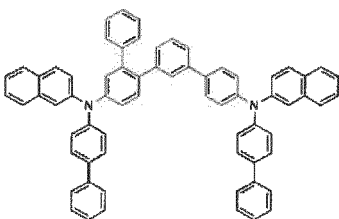
[Chemical Formula 46]
