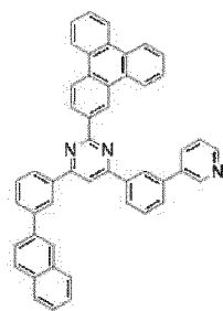
[Chemical Formula 120]
