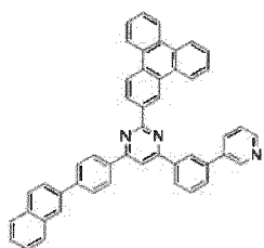
[Chemical Formula 107]
