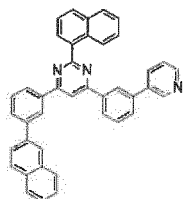
[Chemical Formula 115]
