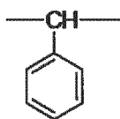
[Chemical Formula 15]
