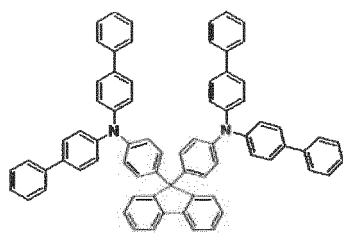
[Chemical Formula 215]
