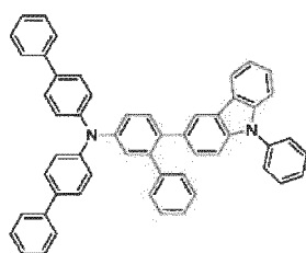
[Chemical Formula 76]
