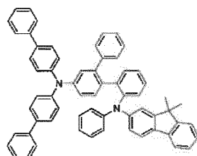
[Chemical Formula 75]
