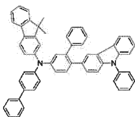
[Chemical Formula 65]
