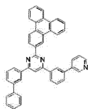
[Chemical Formula 89]
