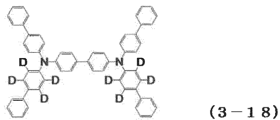
[Chemical Formula 221]
