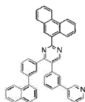
[Chemical Formula 137]
