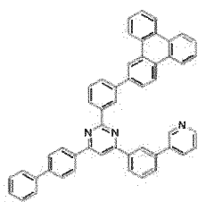
[Chemical Formula 194]
