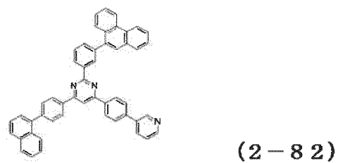
[Chemical Formula 158]
