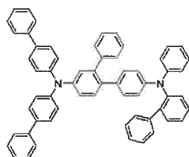
[Chemical Formula 70]
