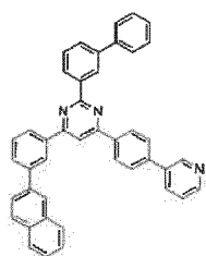
[Chemical Formula 173]
