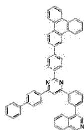
[Chemical Formula 183]
