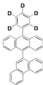
[Chemical Formula 257]
