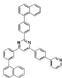
[Chemical Formula 168]
