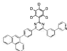
[Chemical Formula 121]
