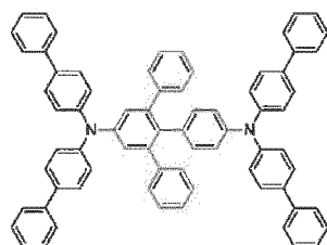
[Chemical Formula 76]
