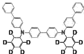
[Chemical Formula 218]
