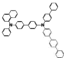
[Chemical Formula 217]
