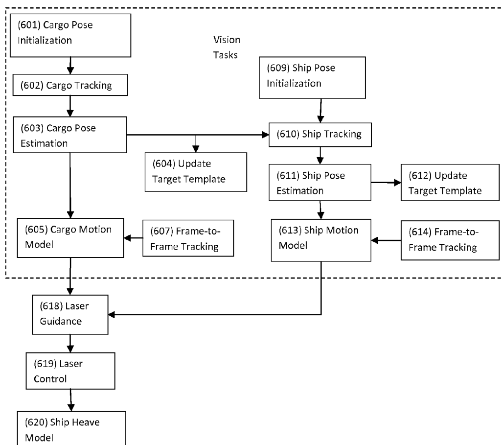
Fig. 16 - Flow chart Overview of the 3D model based tracking of the cargo
