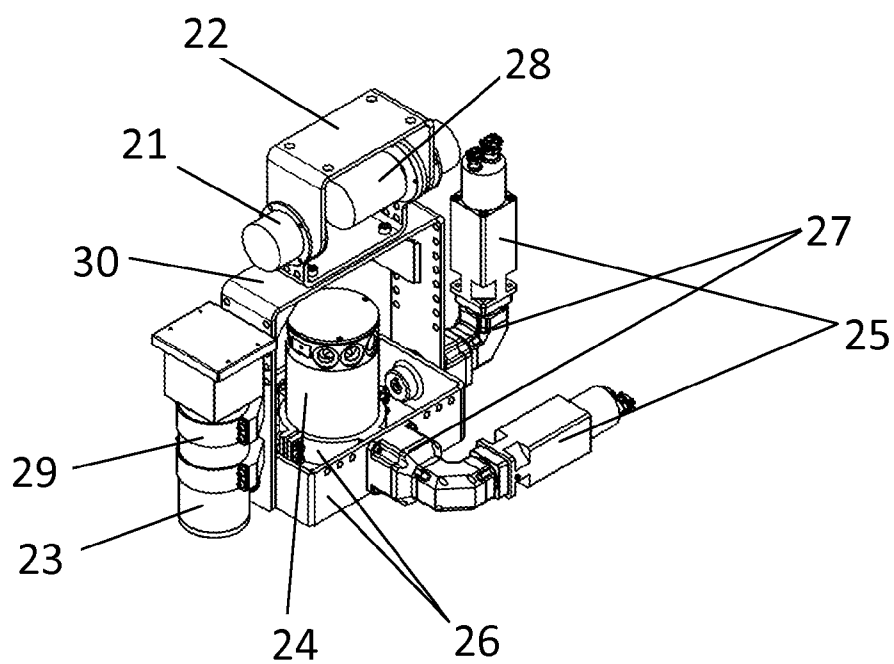
Figure 4 – One embodiment of Sensor platform
