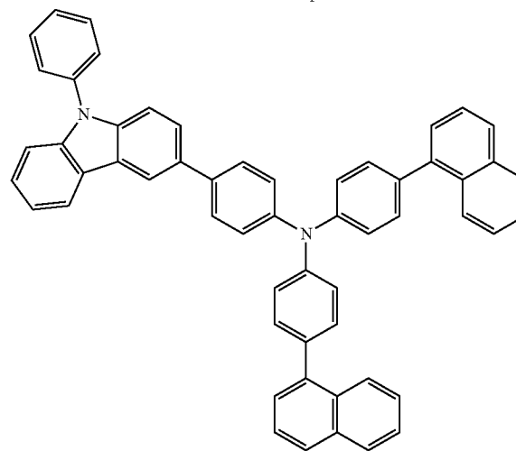
PCBNBB
