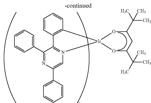
[Ir(tppr) 2 (dpm)]
