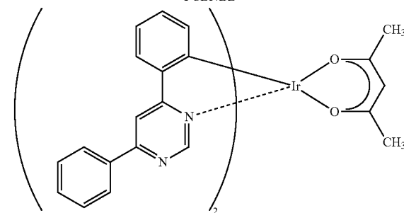
[Ir(dppm) 2 (acac)]
