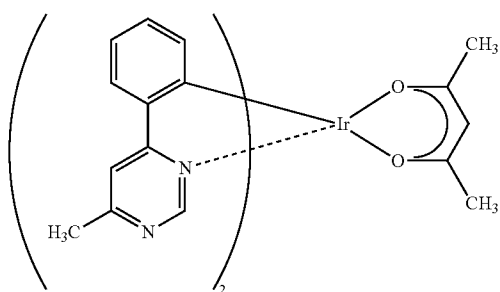
[Ir(mppm) 2 (acac)]
