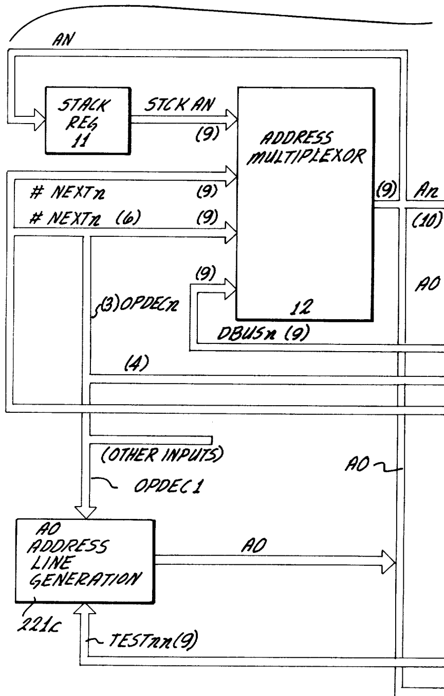
FIG. 5A-1: BLOCK DIAGRAM FOR ON-LINE OPERATION
