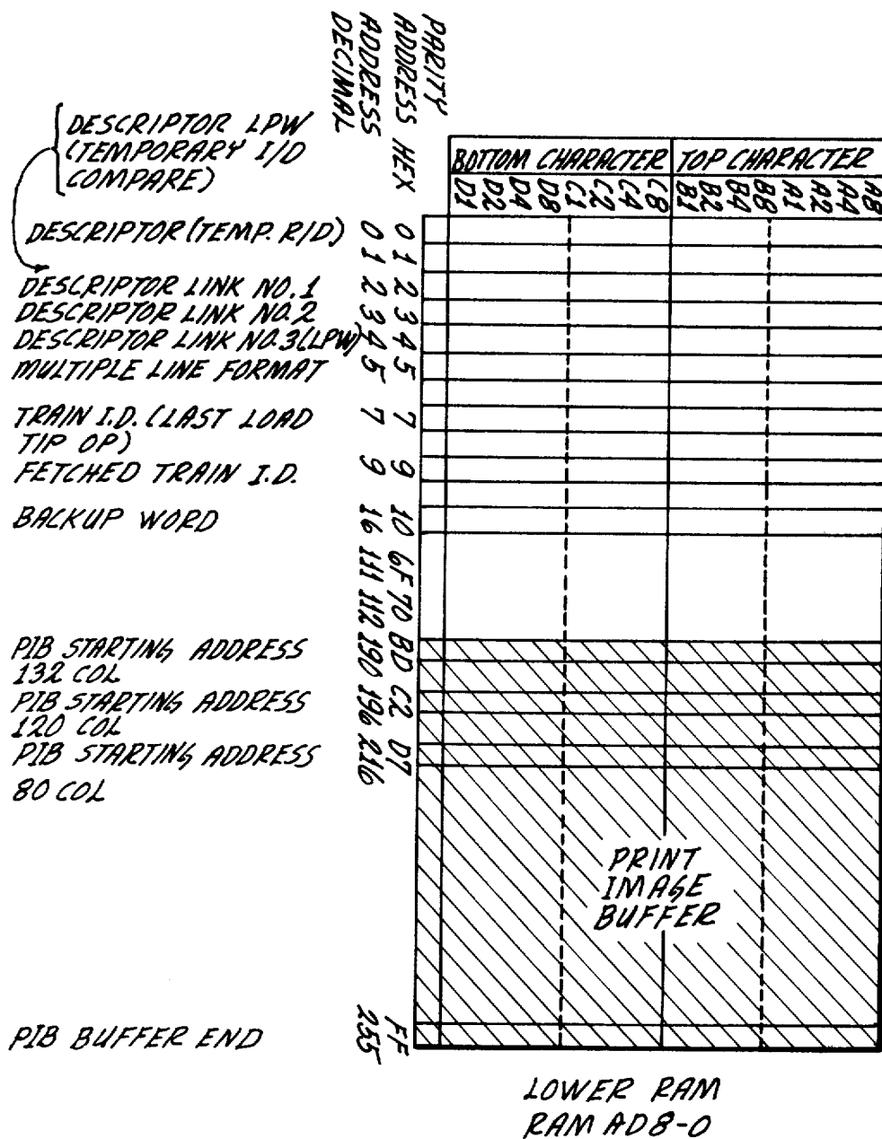
F14.5C-1 MEMORY USAGE
