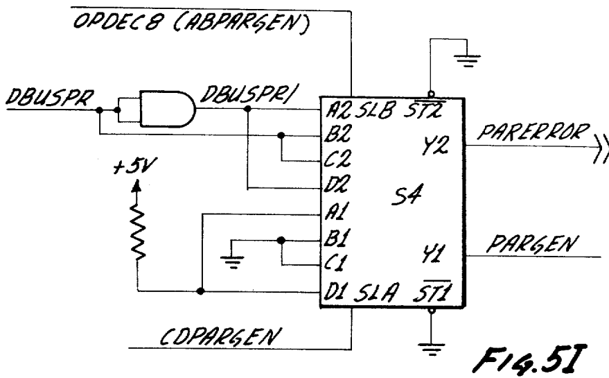
VERTICAL PARITY GENERATION/ CHECK
