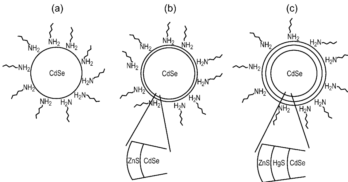
DIAGRAM OF a) CORE PARTICLE, b) CORE-SHELL PARTICLE, c) CORE-MULTI SHELL ORGANIC CAPPED PARTICLE
