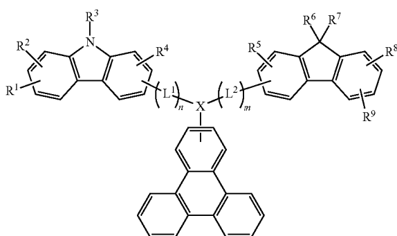
[Chemical Formula 5]
