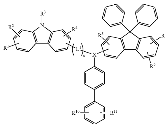
[Chemical Formula 6]
