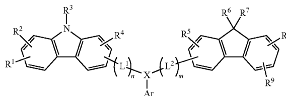
[Chemical Formula 1]
