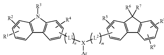
[Chemical Formula 2]
