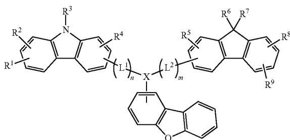
[Chemical Formula 3]
