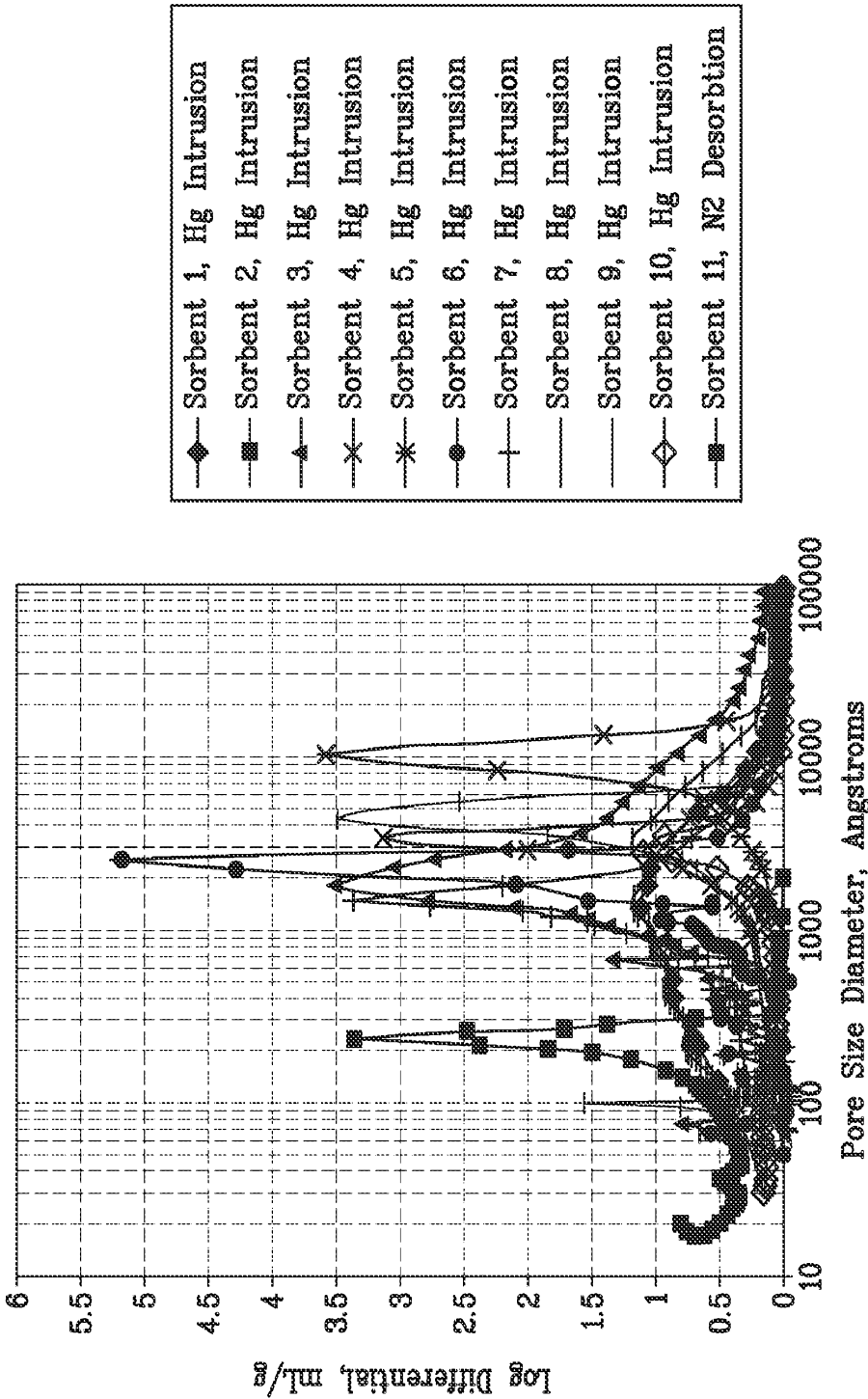
Plot of pore volume as a function of the pore diameter
