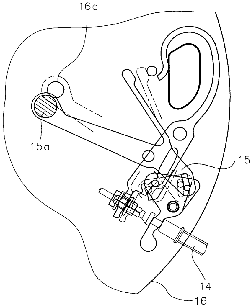
FIG. 6 PRIOR ART
