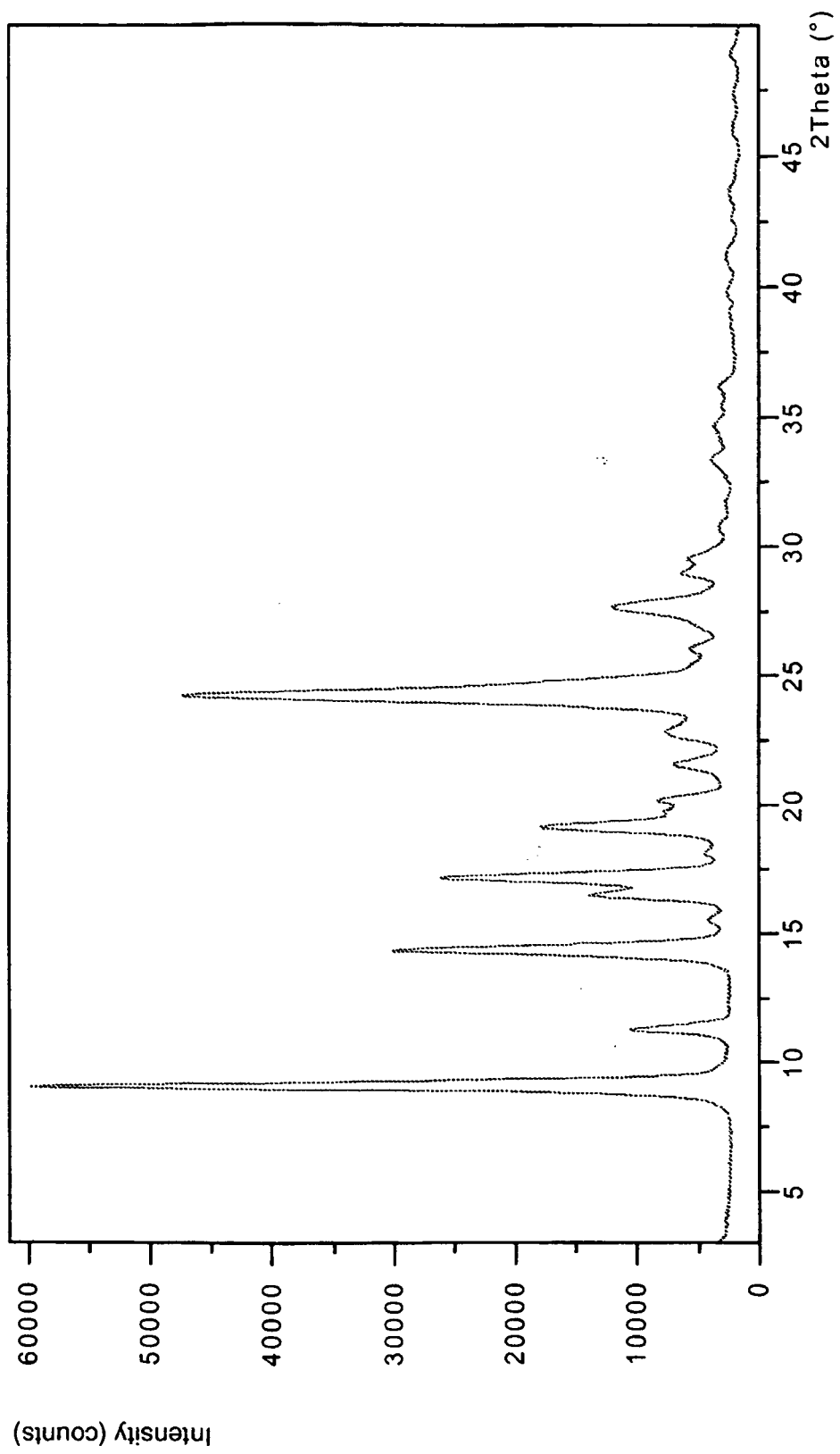
Figure 2: Powder XRD pattern of TMC278 polymorph I.
