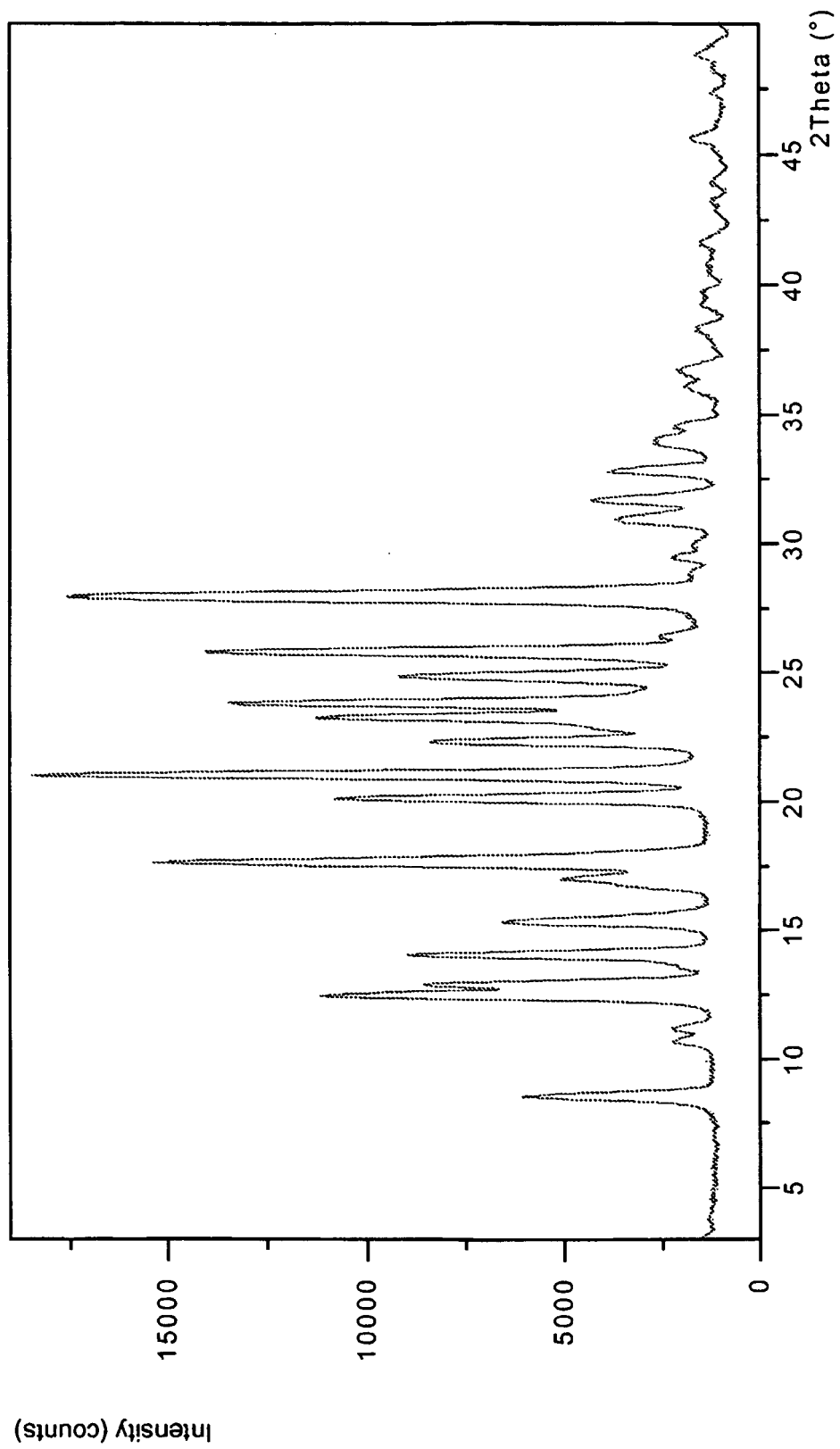
Figure 6: Powder XRD pattern of TMC278 polymorph II.
