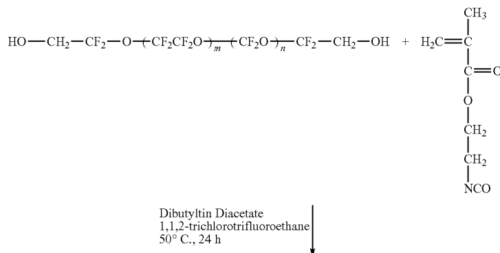
Scheme 1. Synthesis and Photocuring of Functional Perfluoropolyethers.
