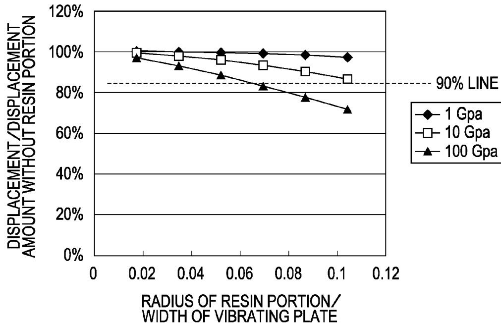
RADIUS AND DISPLACEMENT AMOUNT OF RESIN PORTION
