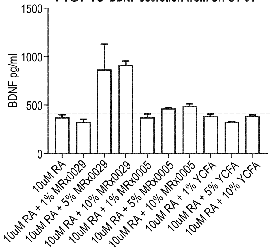
FIG. 19 BDNF secretion from SH-SY-5Y
