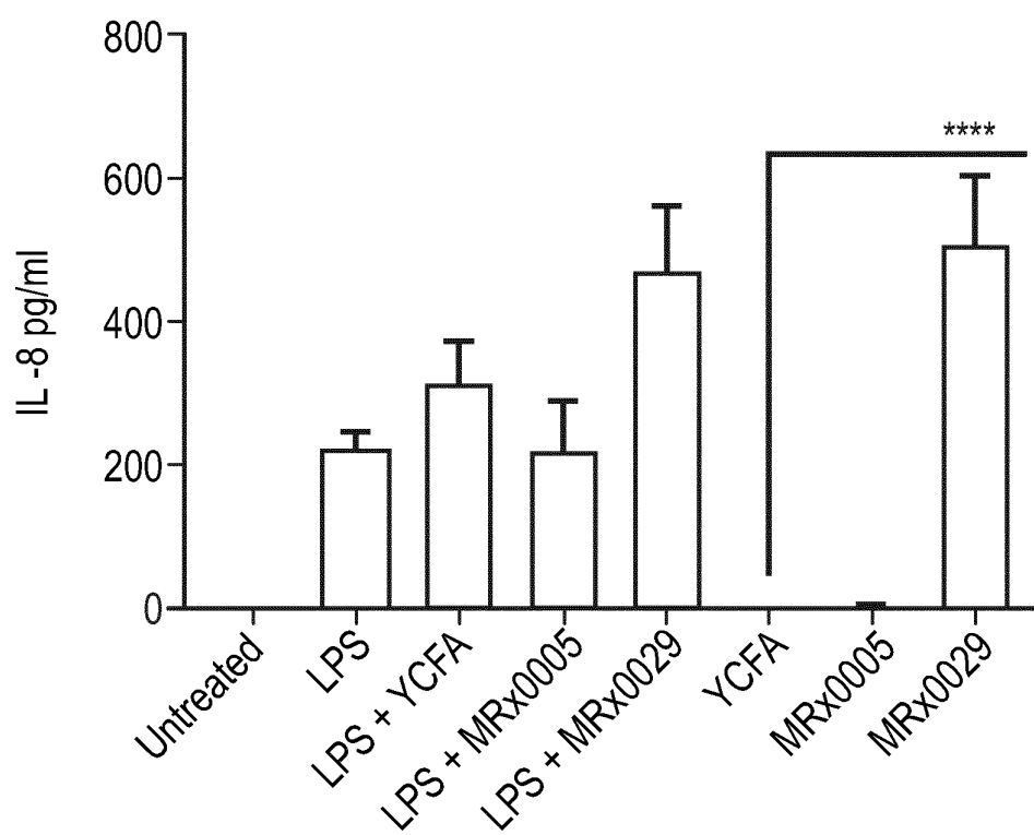
FIG. 3 Secretion of IL-8 from U373
