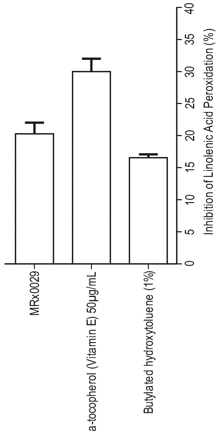
FIG. 8 Total Antioxidant Capacity
