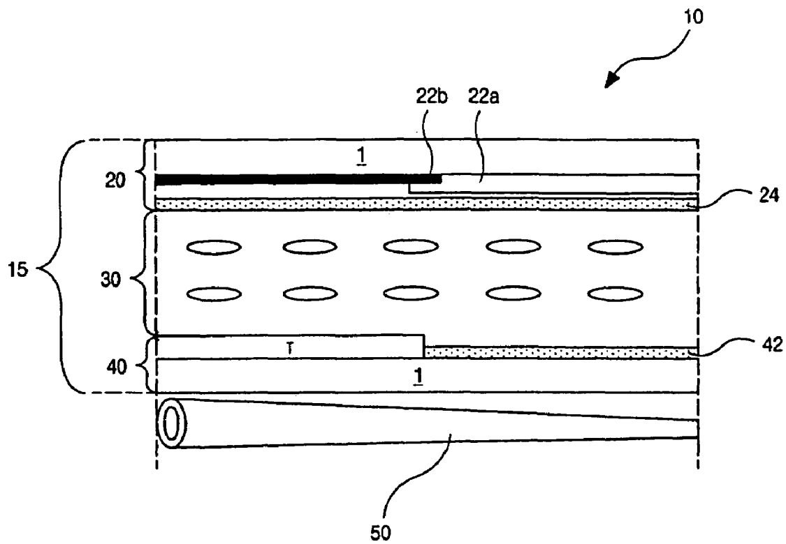
FIG. 1 (RELATED ART)
