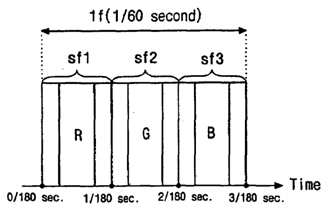
FIG. 5 (RELATED ART)
