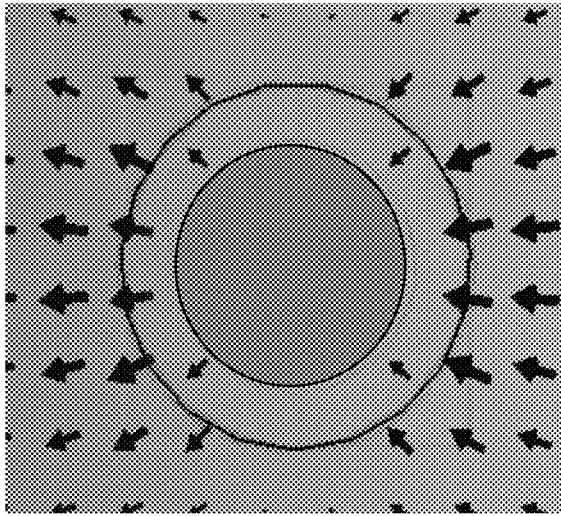
Hybrid mode (HE11) 2157
