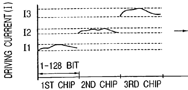
FIG. 16 (PRIOR ART)
