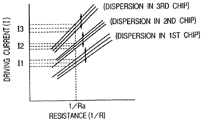
FIG. 17 (PRIOR ART)
