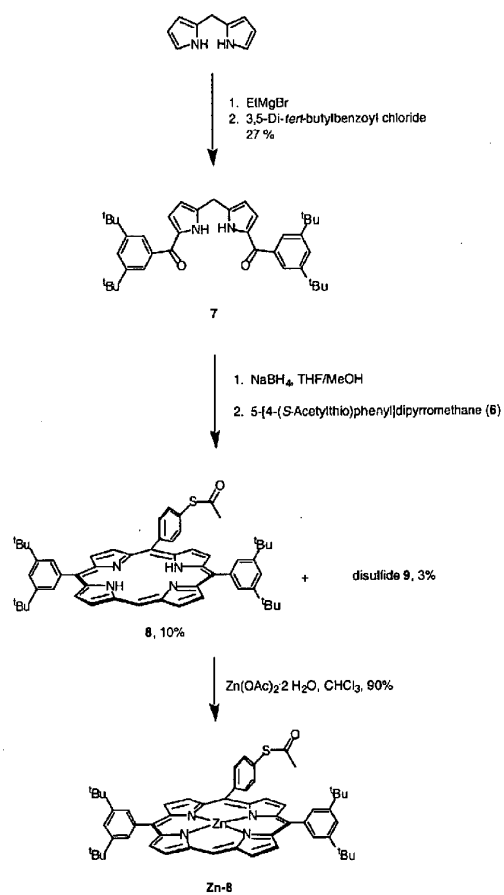
Scheme 3
