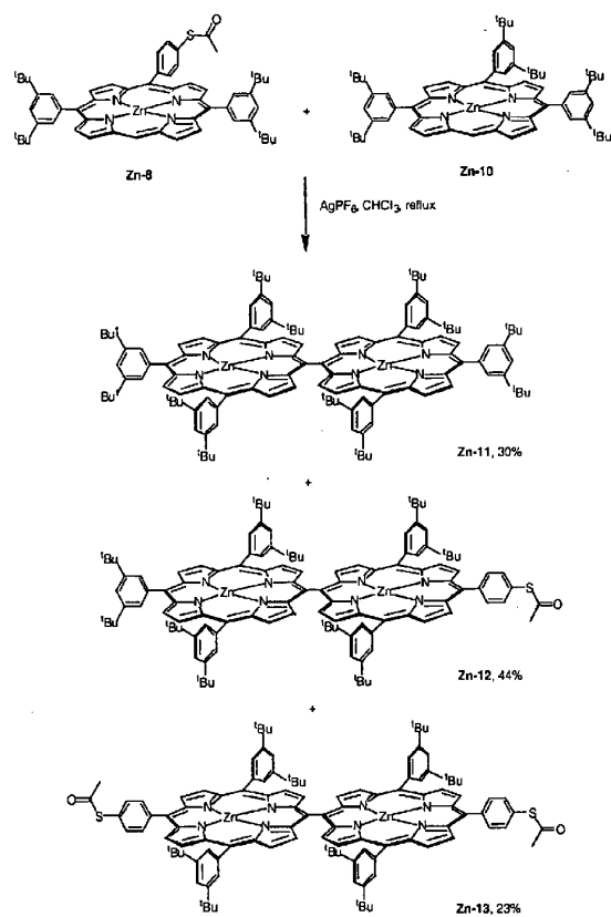
Scheme 6
