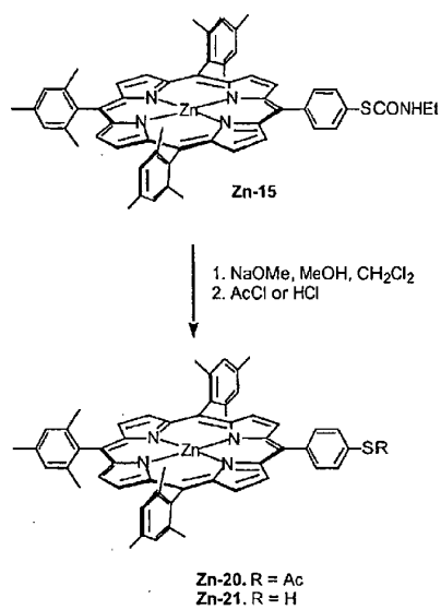
Scheme 4.
