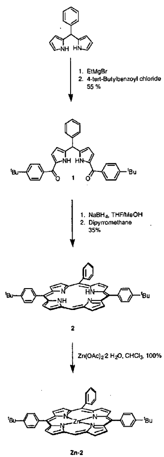
Scheme 1
