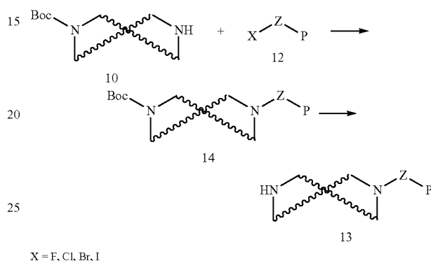
Scheme 6
