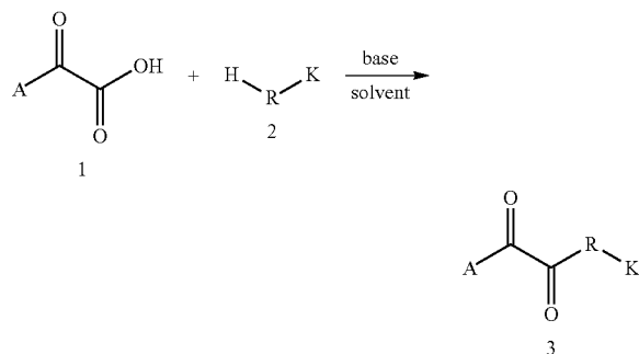
Scheme 1b
