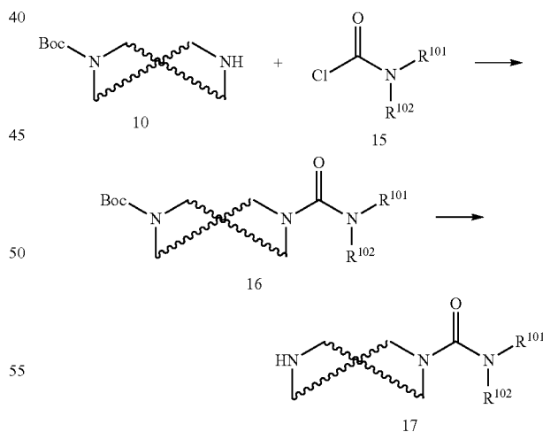
Scheme 7
