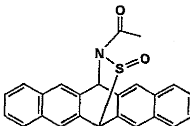
Pentacene precursor
