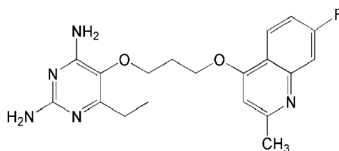
2,4-diamino-6-ethyl-5-(3-(7-fluoro-2-methylquinolin-4-yloxy)propoxy)pyrimidine (P157) ;
