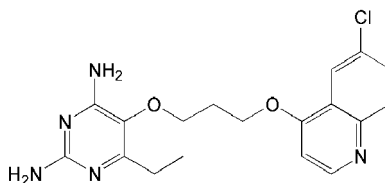
2,4-diamino-6-ethyl-5-(3-(6-chloro-quinolin-4-yloxy)propoxy)pyrimidine (P149) ;
