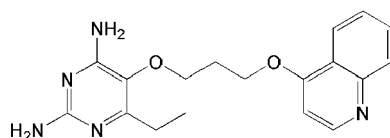
2,4-diamino-6-ethyl-5-(3-(quinolin-4-yloxy)propoxy)pyrimidine (P113);
