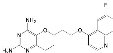
2,4-diamino-6-ethyl-5-(3-(6-fluoro-quinolin-4-yloxy)propoxy)pyrimidine (P153);
