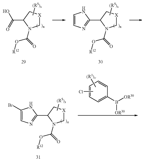
Scheme 7: Heteroaryls
