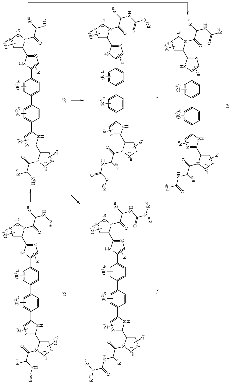
Scheme 4: Symmetric Biphenyls
