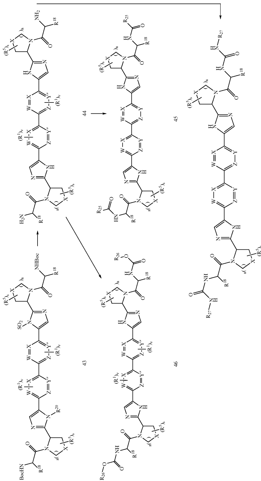
Scheme 10: Starting Material 29
