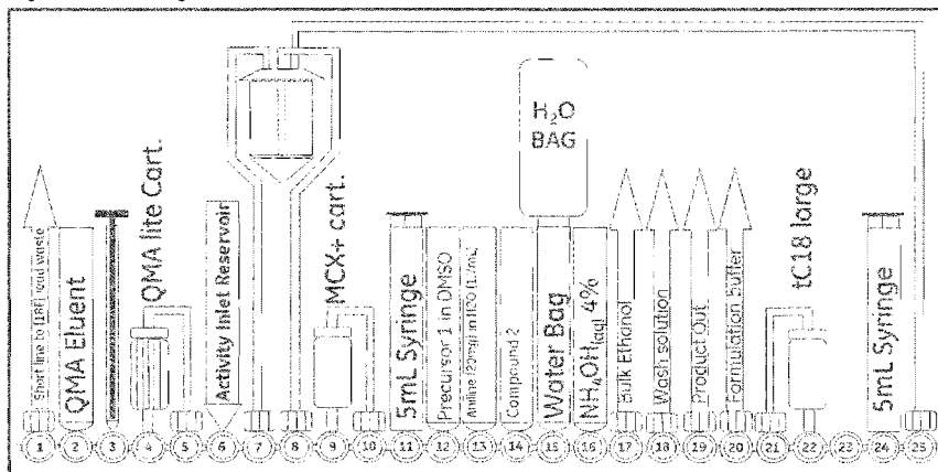
Figure 2: Cassette Configuration.
