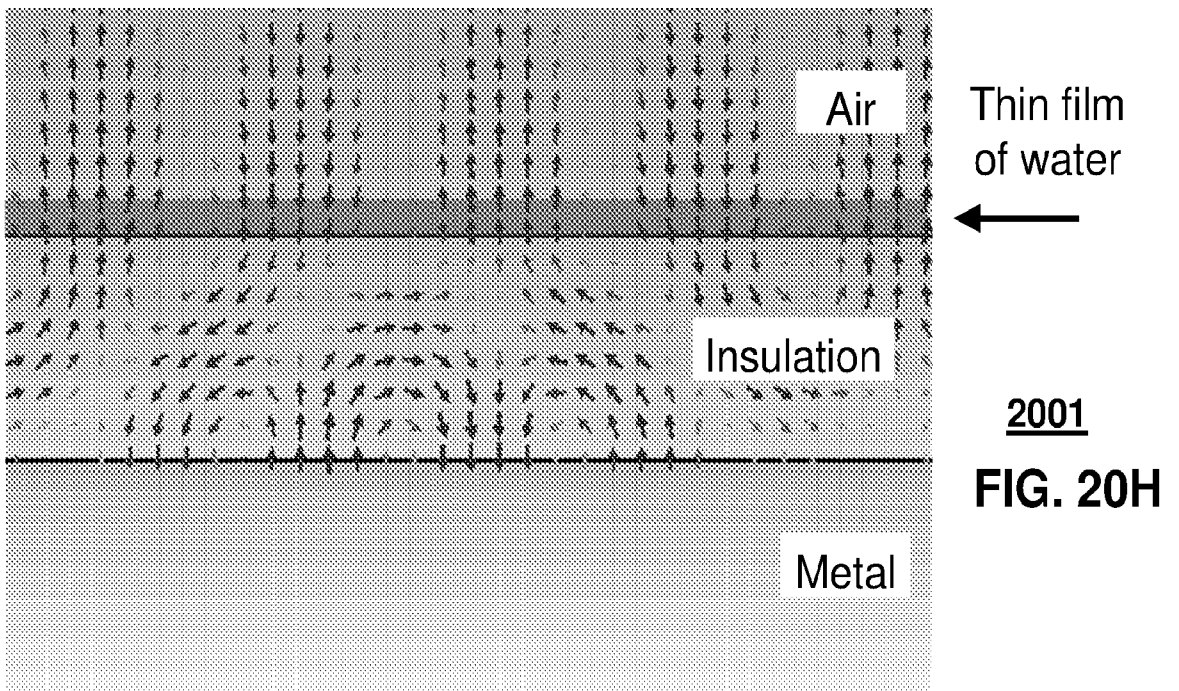
Longitudinal Section of Cable showing e-fields of TM 01 waves at 40 GHz
