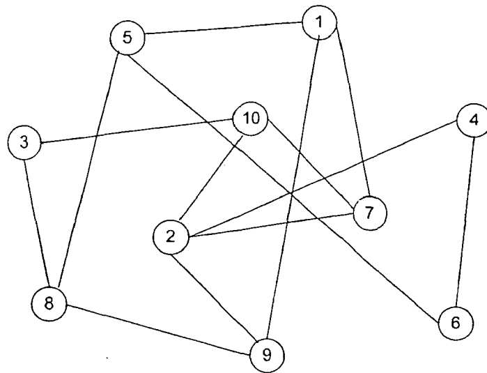
Figure 3. Simple Graph
