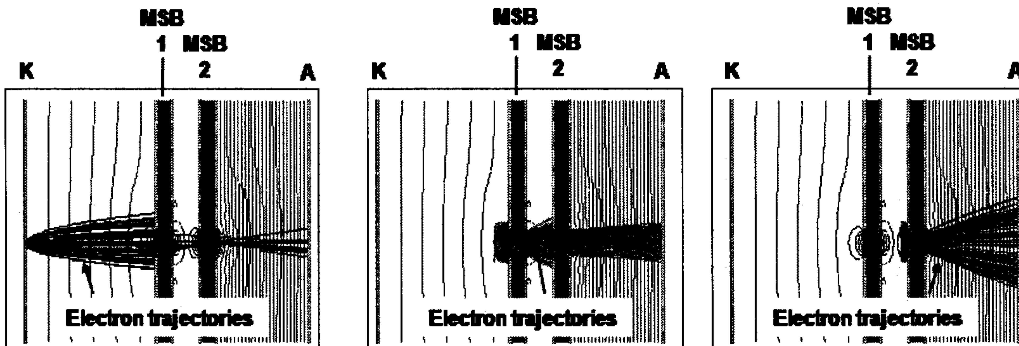
Fig 2 a) Primary electrons from the photo-cathode (K) strike the MSB 1, releasing secondary electrons. A small fraction of primary electrons pass through the MSB 1 holes. Equipotential lines are also illustrated, running approximately parallel to the conductive surfaces.
