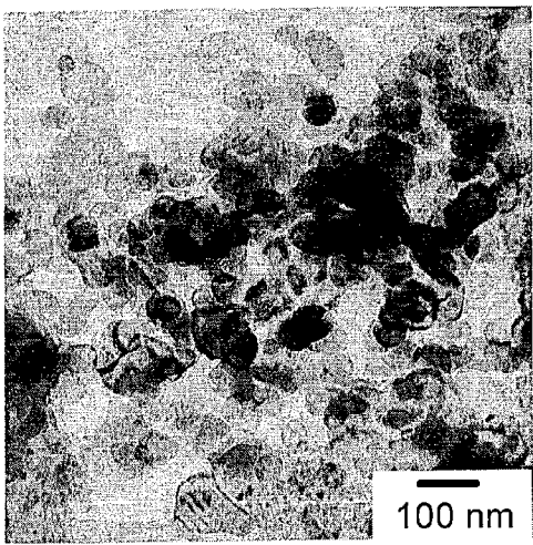
1 % Nb doped
