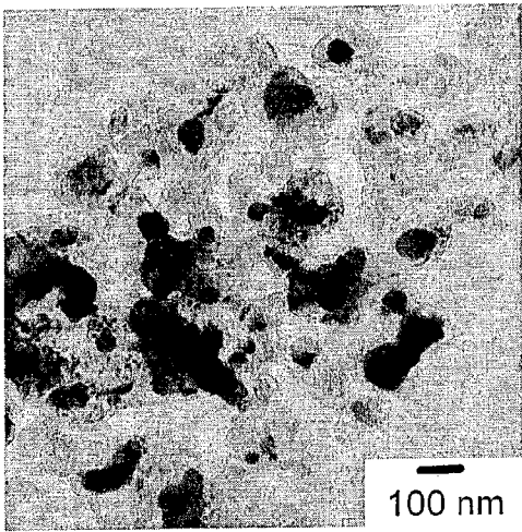
1 % Zr doped
