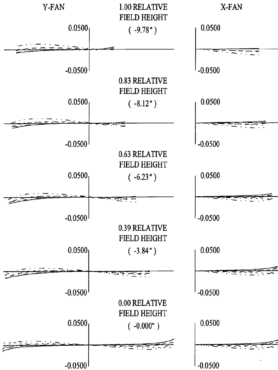
Fig. 43 RAY ABERRATIONS (MILLIMETERS) POSITION 5 ----- 643.8469 NM ----- 587.5600 NM ----- 546.0700 NM ----- 486.1300 NM ----- 460.0000 NM
