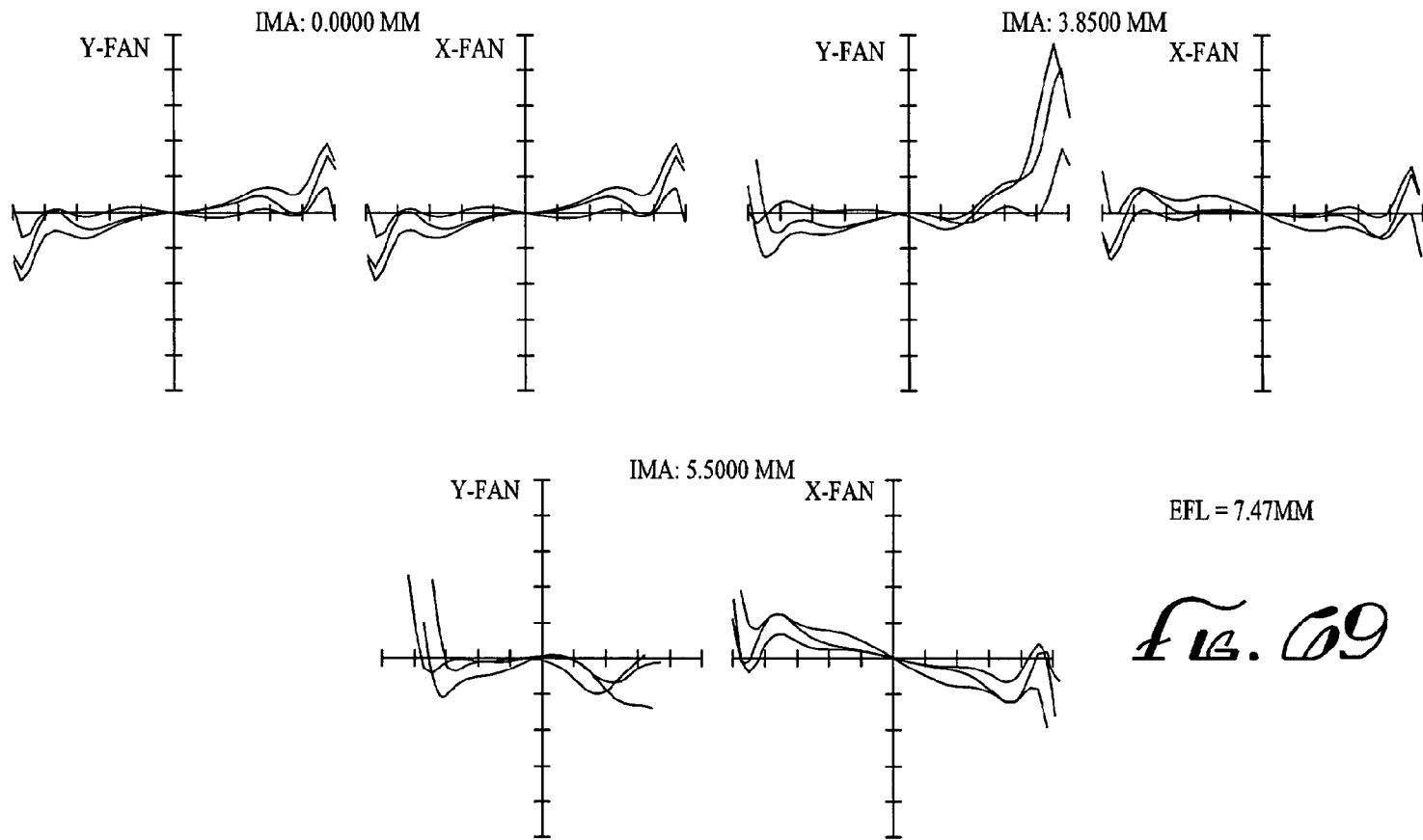
WAVE LENGTHS RANGE 480-644 NM MAXIMUM VERTICAL SCALE +/- 100 MICRONS
