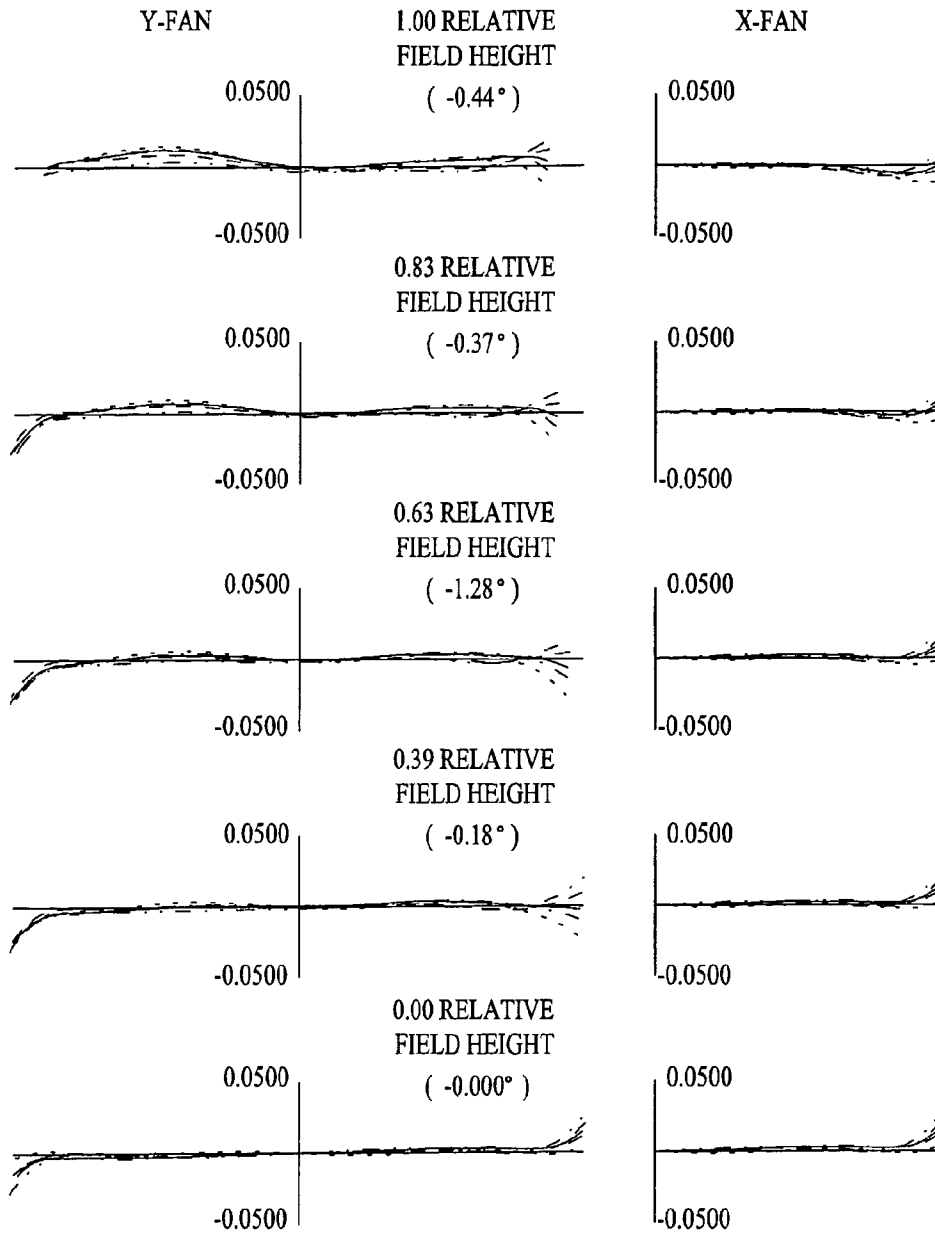
Fig. 49 RAY ABERRATIONS (MILLIMETERS) POSITION 11 ----- 643.8469 NM ----- 587.5600 NM ----- 546.0700 NM ----- 486.1300 NM ----- 460.0000 NM
