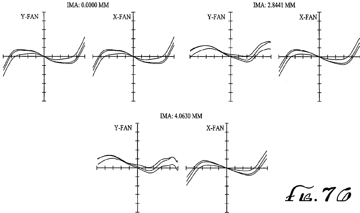
WAVELENGTH RANGE 8-12 MICRONS MAXIMUM VERTICAL SCALE +/- 200 MICRONS
