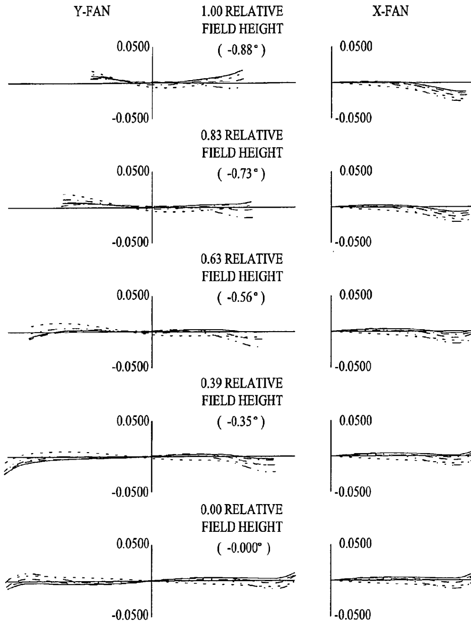
Fig. 4B RAY ABERRATIONS (MILLIMETERS) POSITION 10 ..... 643.8469 NM ----- 587.5600 NM ———— 546.0700 NM - - - - 486.1300 NM - . - . 460.0000 NM
