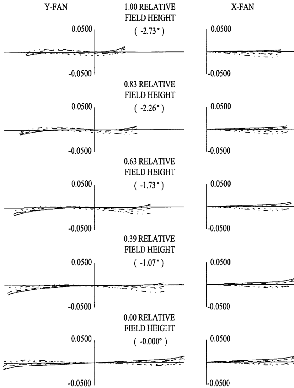
Fig. 57 RAY ABERRATIONS (MILLIMETERS) POSITION 19 ----- 643.8469 NM ----- 587.5600 NM ----- 546.0700 NM ----- 486.1300 NM ----- 460.0000 NM
