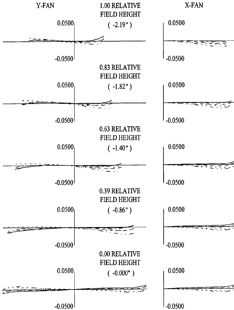
Fig. 40 RAY ABERRATIONS (MILLIMETERS) POSITION 8 ----- 643.8469 NM ----- 587.5600 NM ----- 546.0700 NM ----- 486.1300 NM ----- 460.0000 NM
