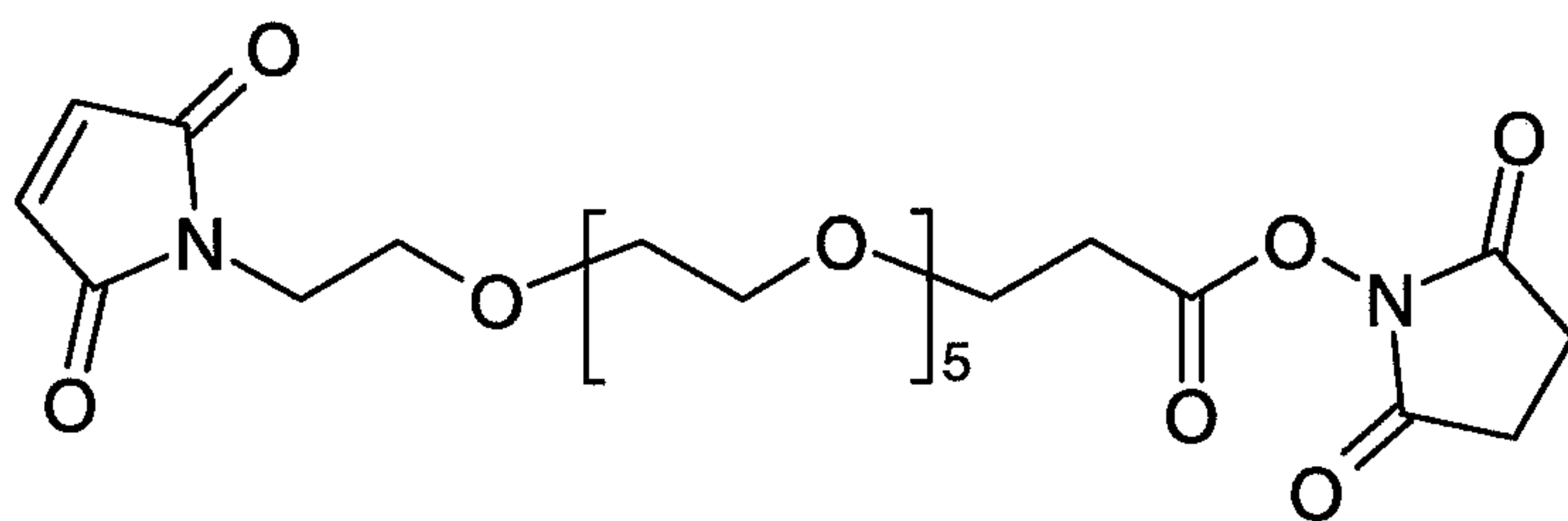
Mal-PEG6-NHS
