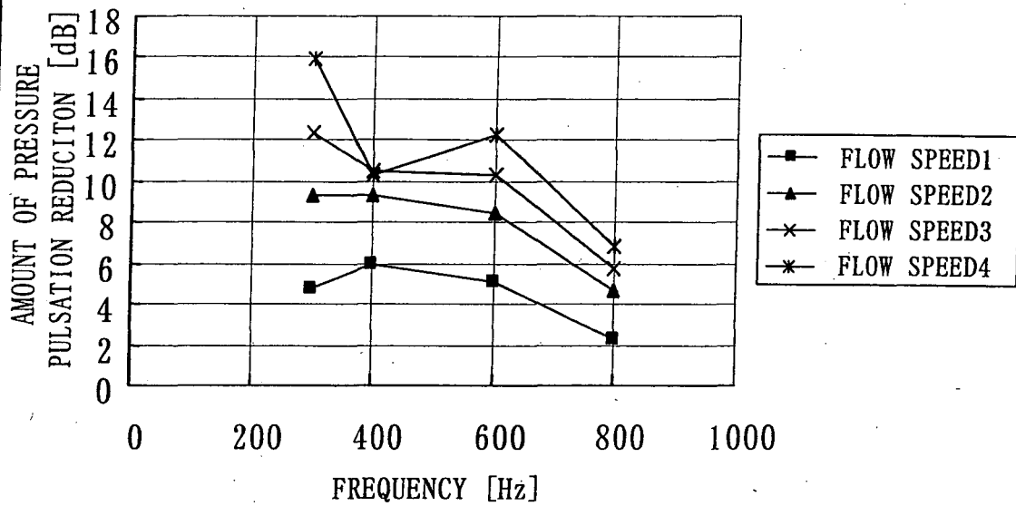
(1) PRESSURE PULSATION REDUCITON OF AIR JET BLOW
