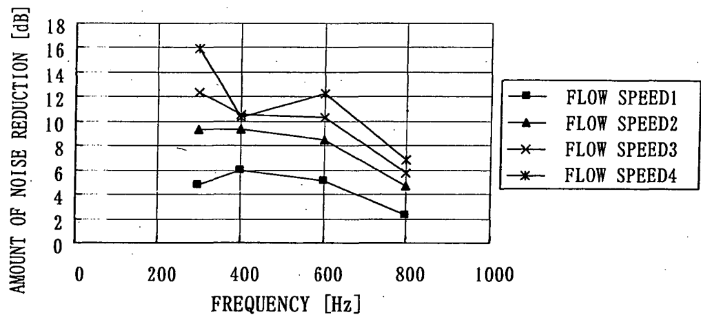
(1) NOISE REDUCTION OF AIR JET BLOW
