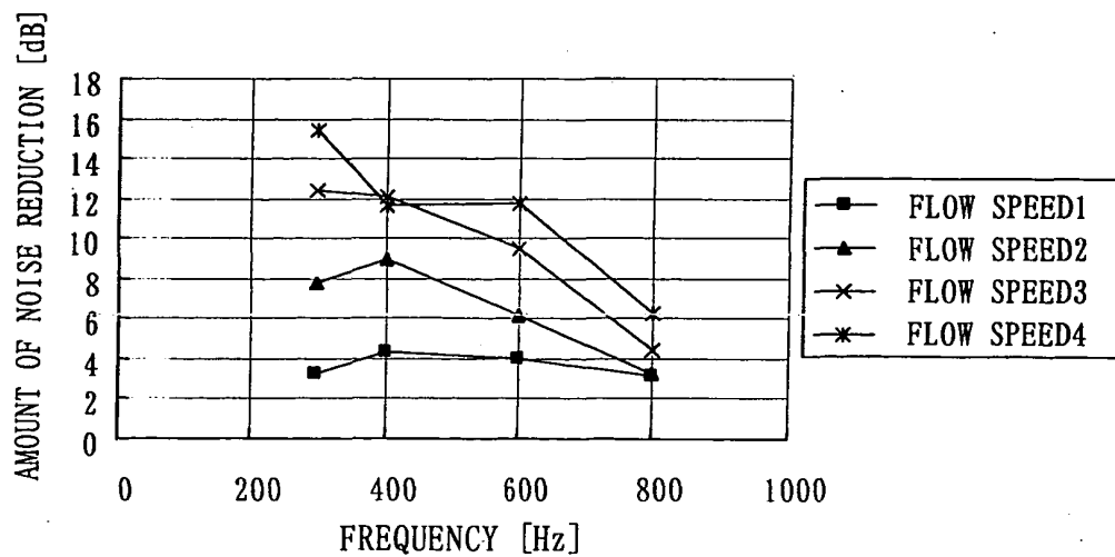
(2) NOISE REDUCTION OF AIR JET SUCTION
