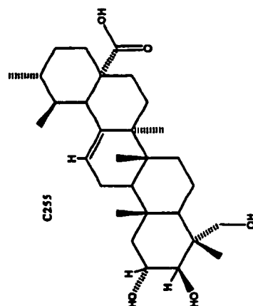
Asiatic acid
