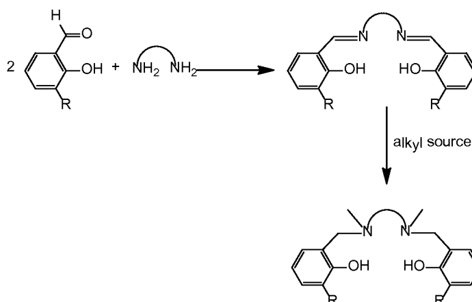
Reaction C:
