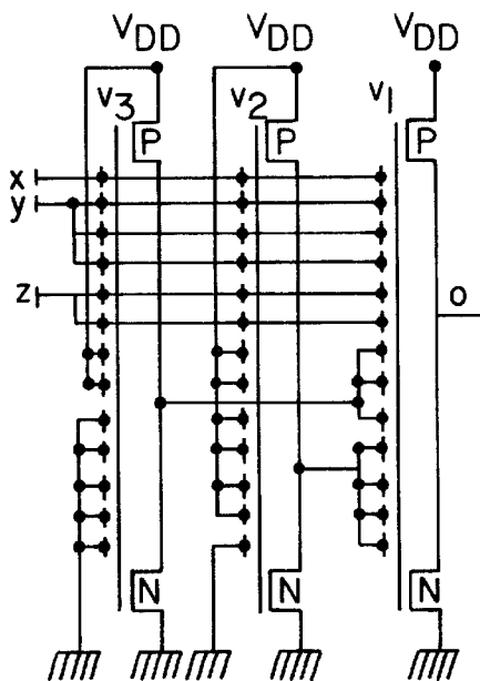
2-stage neuMOS Circuit
