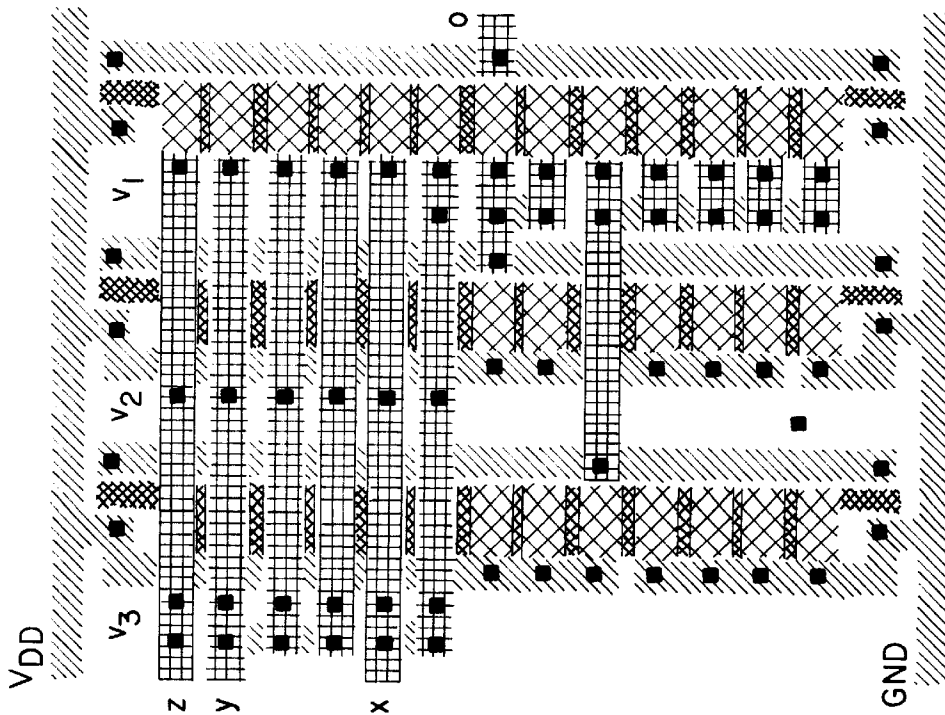
2-stage neuMOS Circuit
