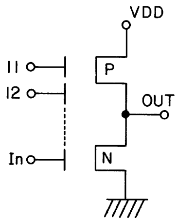
Circuit Symbols
