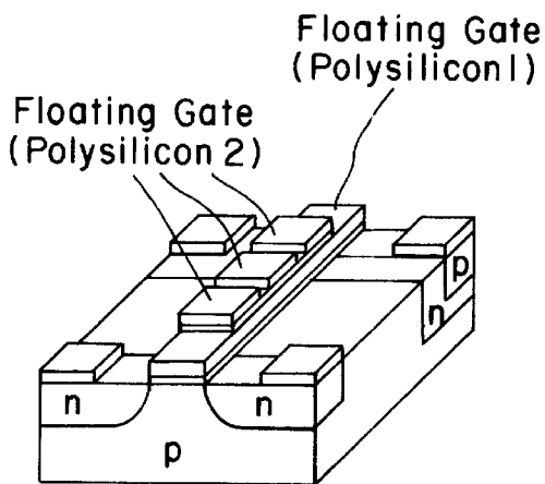
Structural Diagram
