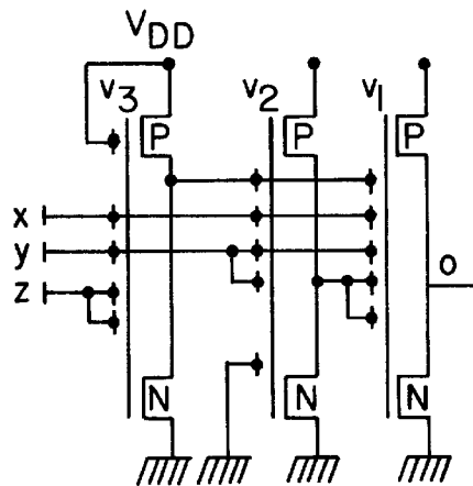
Multi-stage neuMOS Circuit
