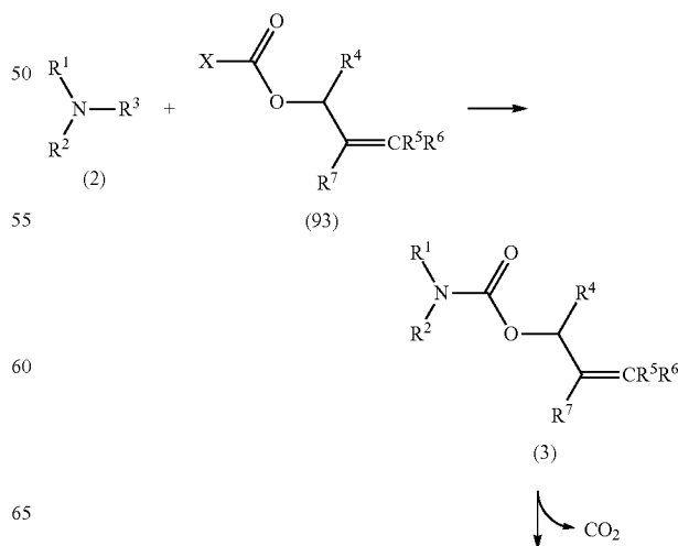
Scheme 30
