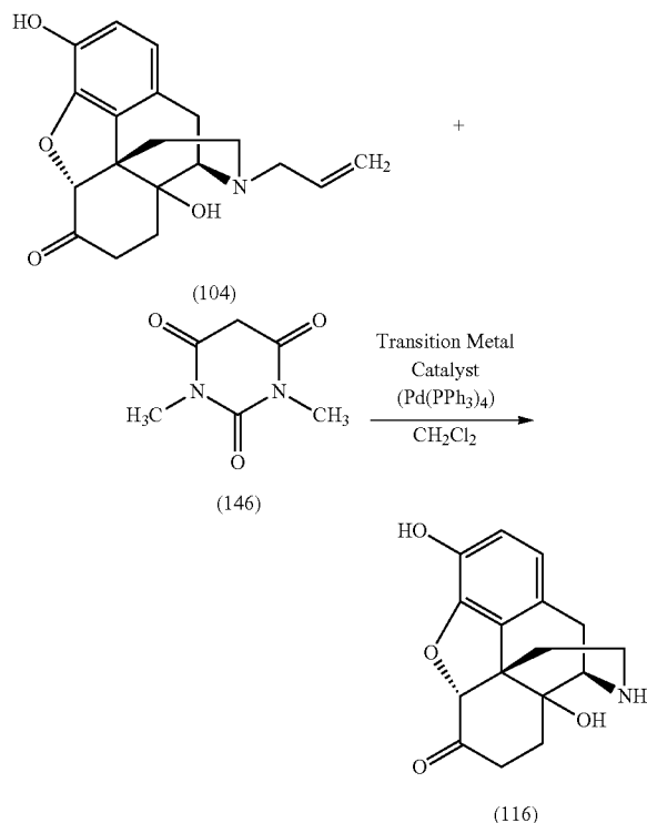
Scheme 14
