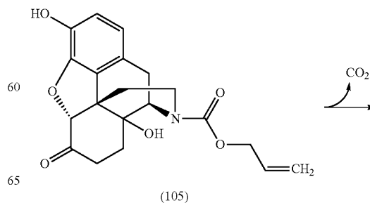
Scheme 5
