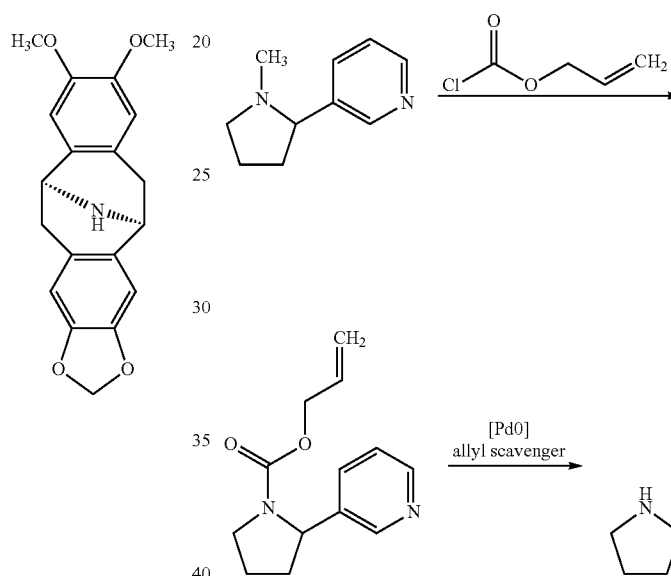
Scheme 28: Nicotine
