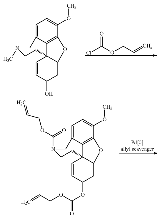
Scheme 27: Galanthamine
