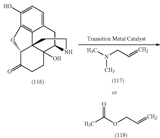
Scheme 13
