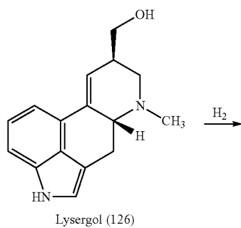
Scheme 19
