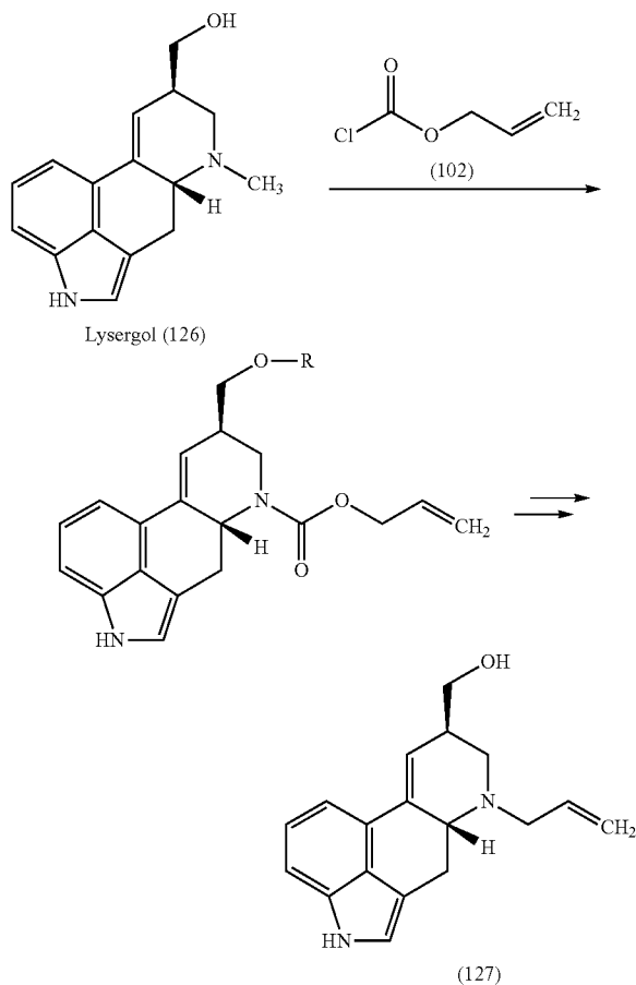
Scheme 17
