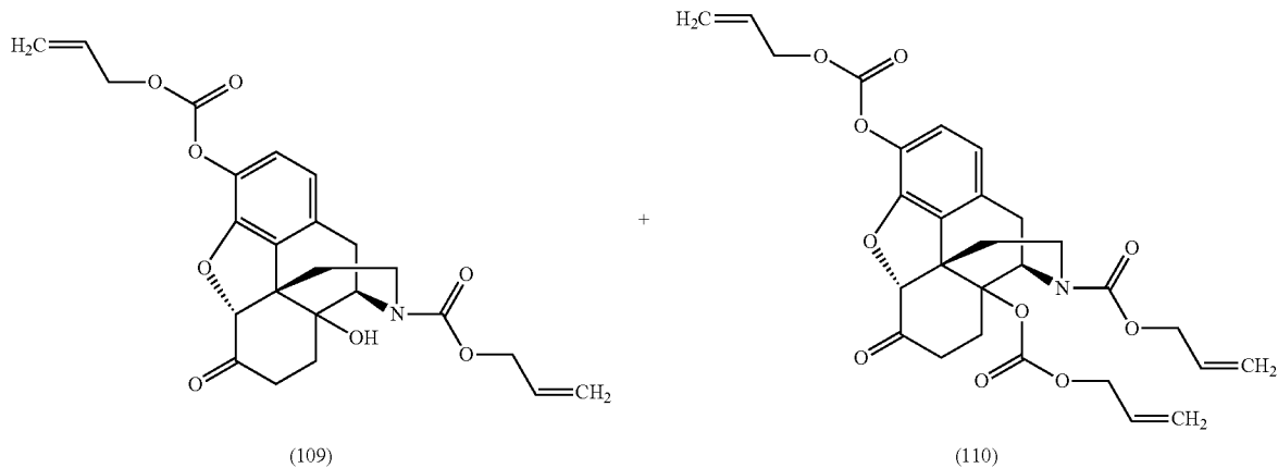
Scheme 7
