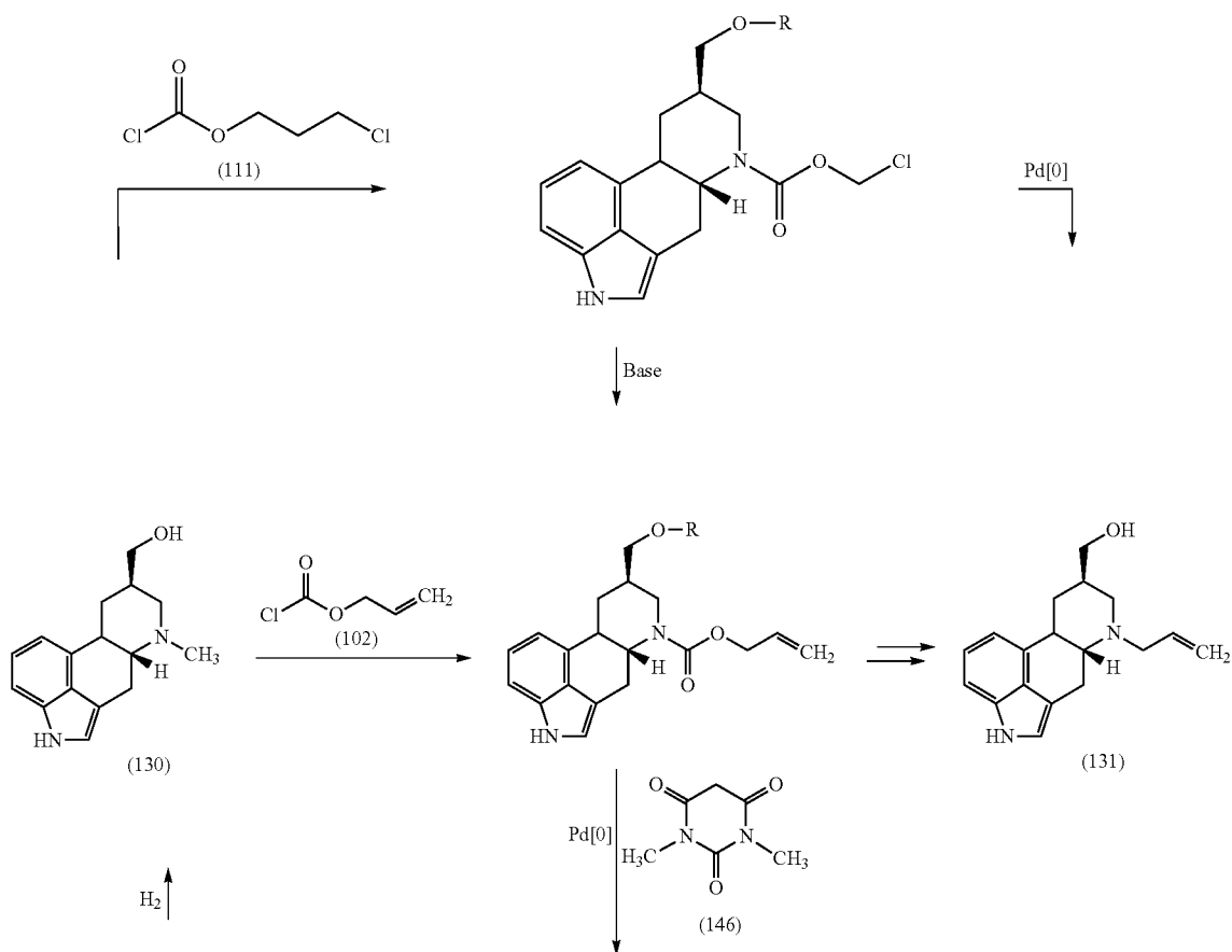
Scheme 20
