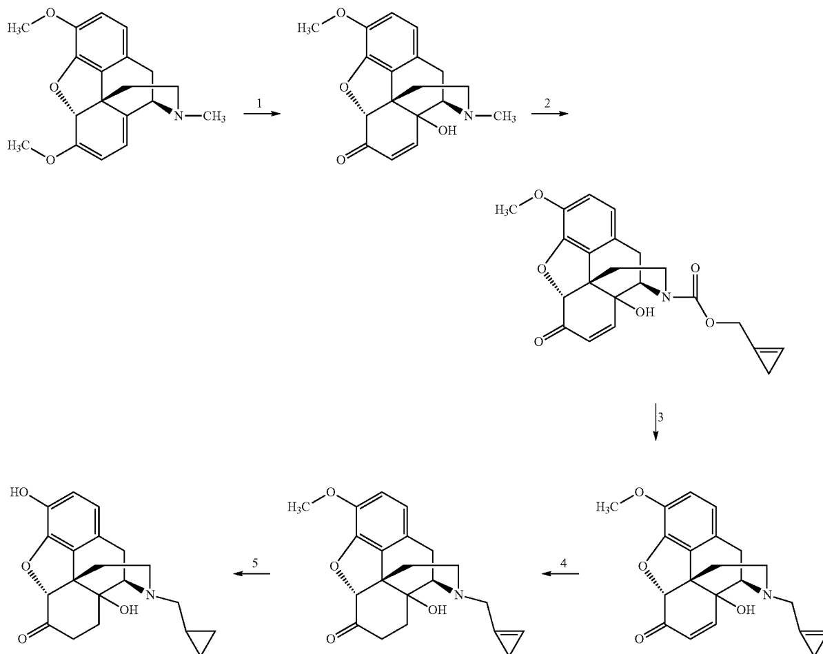
Scheme 34
