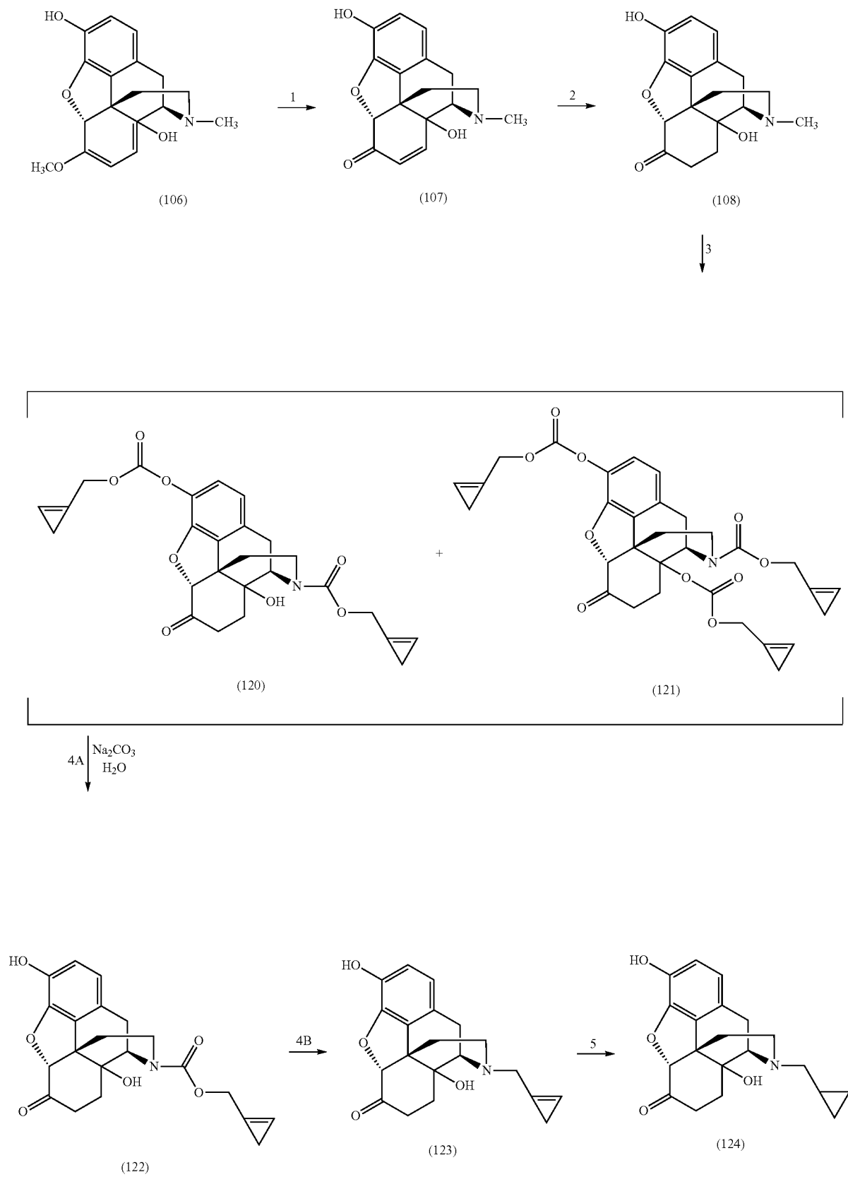
Scheme 16
