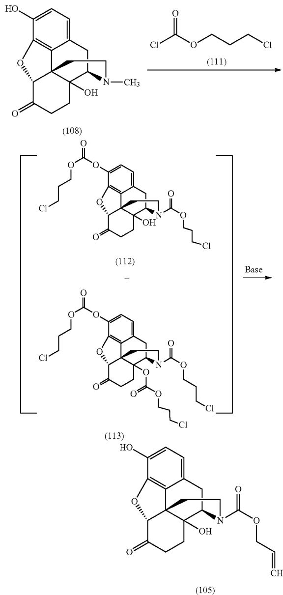
Scheme 11
