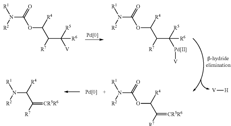
Scheme 29
