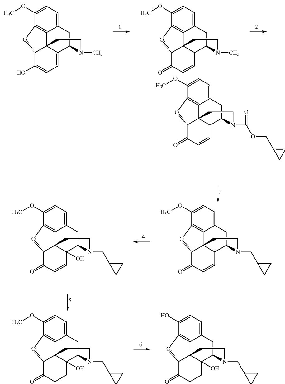
Scheme 33
