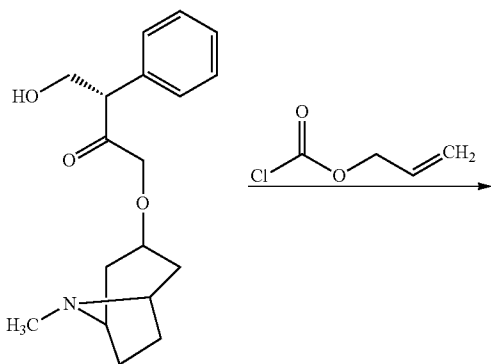
Scheme 24: Atropine
