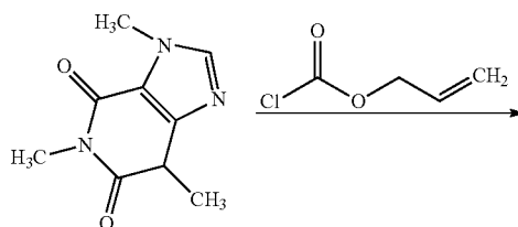
Scheme 25: Caffeine
