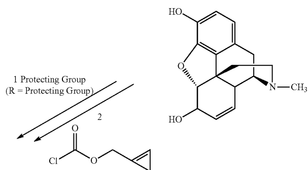
Scheme 32
