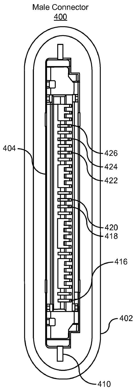
Top View Fig. 4C
