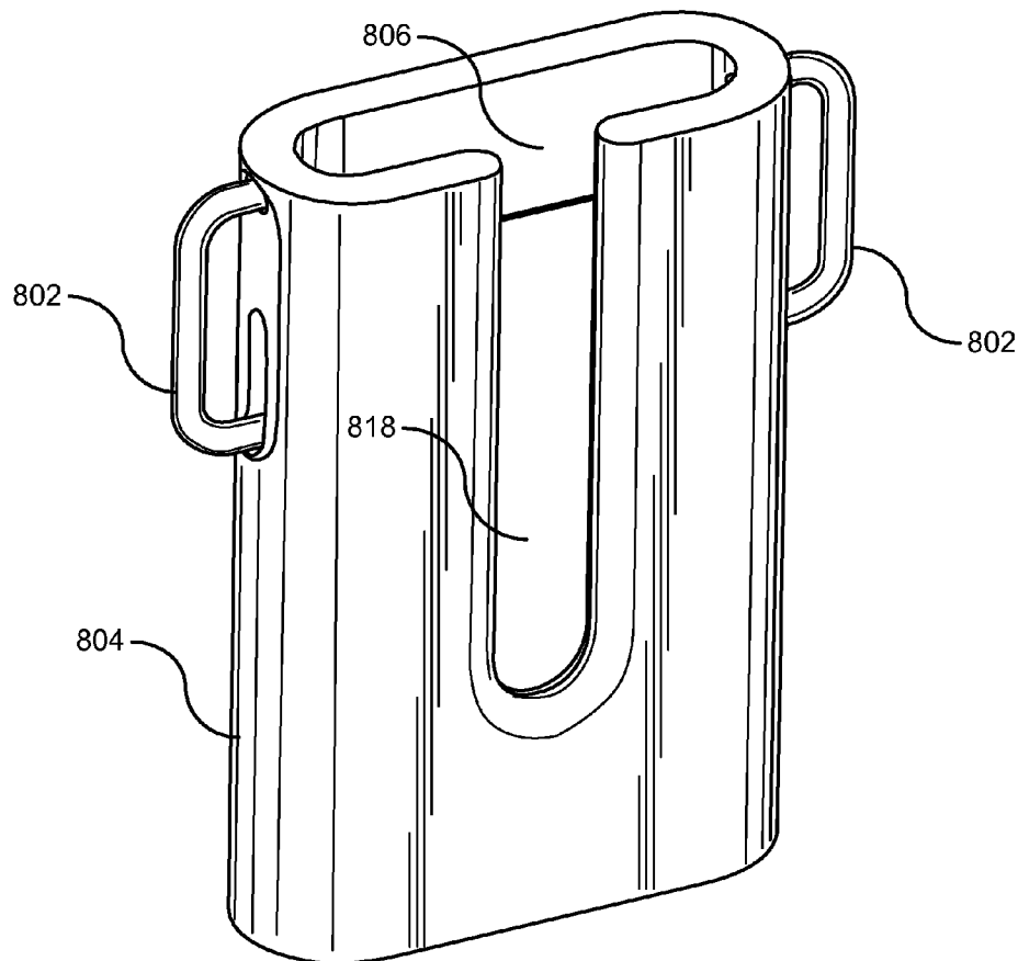
Angled View
