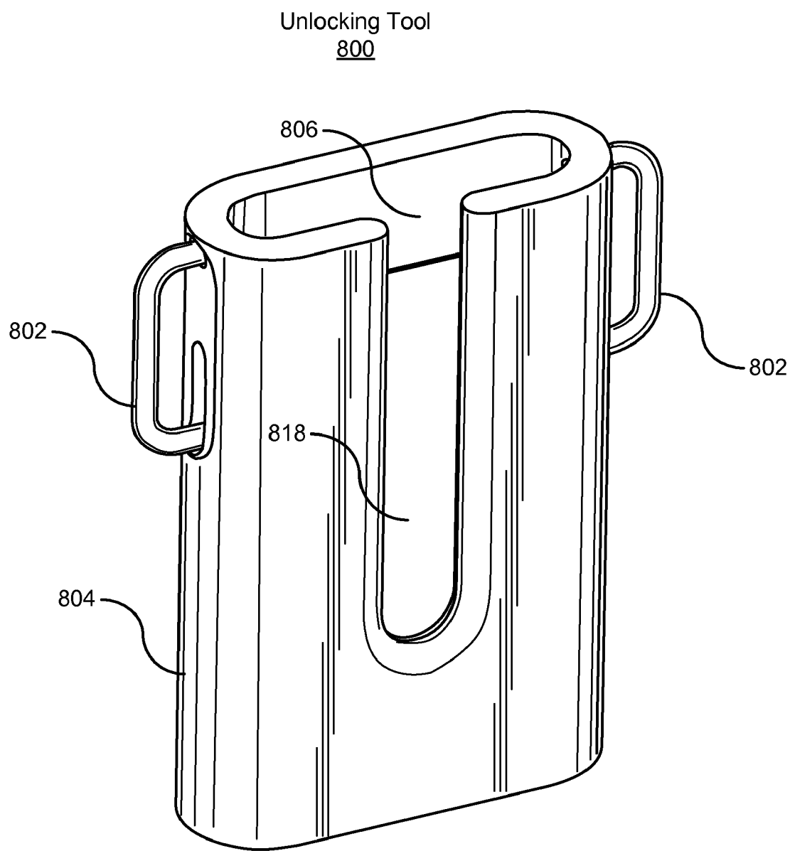
Angled View Fig. 8C
