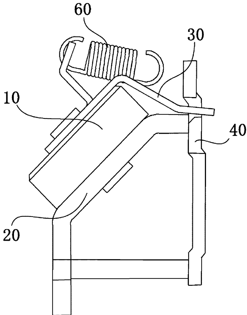
FIG. 1 (PRIOR ART)
