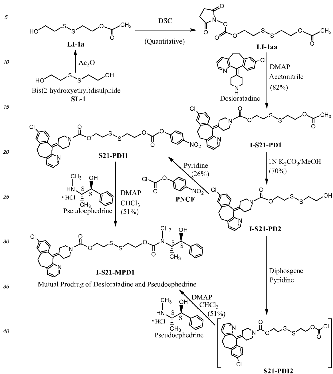
Scheme 21: A Mutual Prodrug of Desloratadine and Pseudoephedrine
