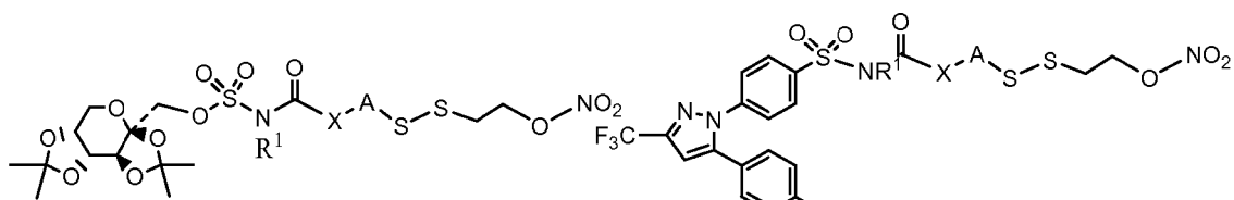
Prodrugs of Topiramate (Anticonvulsant):
