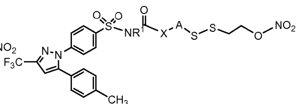
Prodrugs of Celecoxib (Cox-2 Inhibitor):
