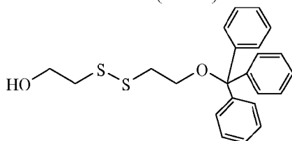
10 2-((2-(Trityloxy)ethyl)disulfanyl)ethanol (LI-1c)
