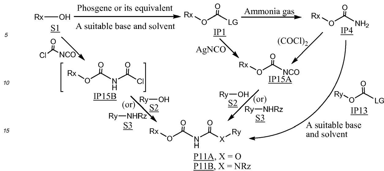
Scheme 8
