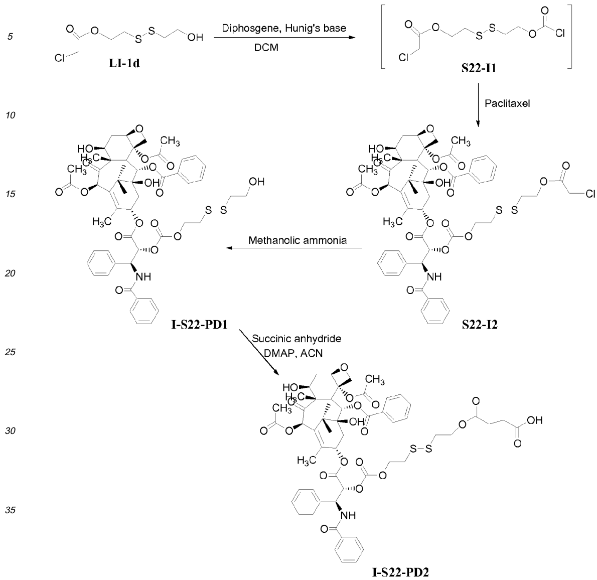
Scheme 22: Synthesis of a water-soluble prodrug of paclitaxel
