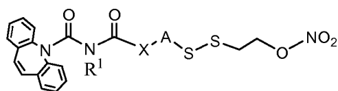
Prodrugs of Carbamazepine (Anticonvulsant):
