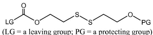
LI-1xy
