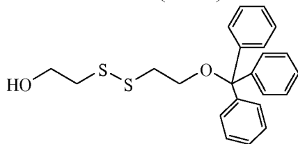
10 2-((2-(Trityloxy)ethyl)disulfanyl)ethanol (LI-1c)
