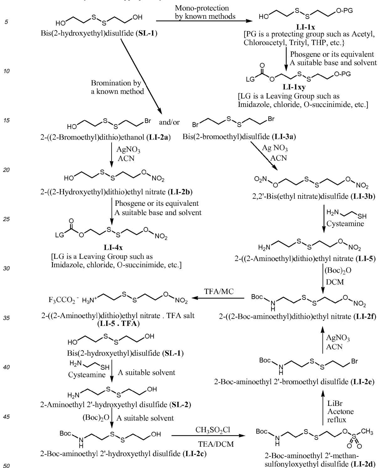
Scheme 10: Synthesis of appropriately derivatized/modified linker intermediates
