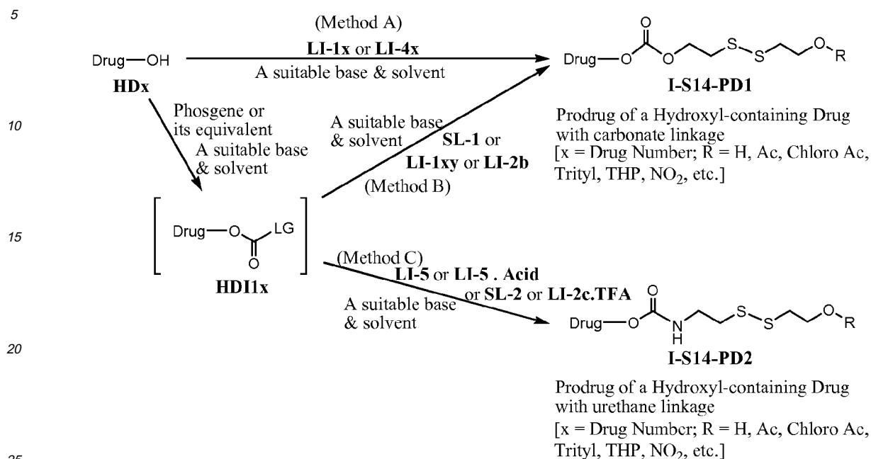
Scheme 14: Synthesis of Prodrugs of Hydroxyl-containing Drugs
