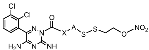
Prodrugs of Lamotrigine (Anticonvulsant):
