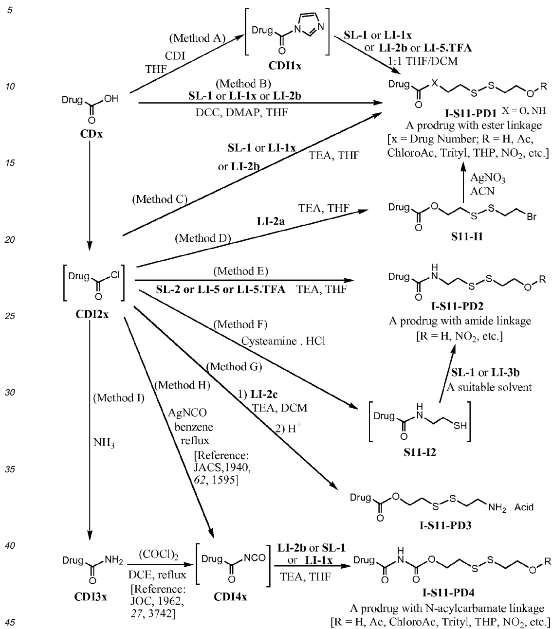
Scheme 11: Synthesis of Prodrugs of Carboxyl-containing Drugs
