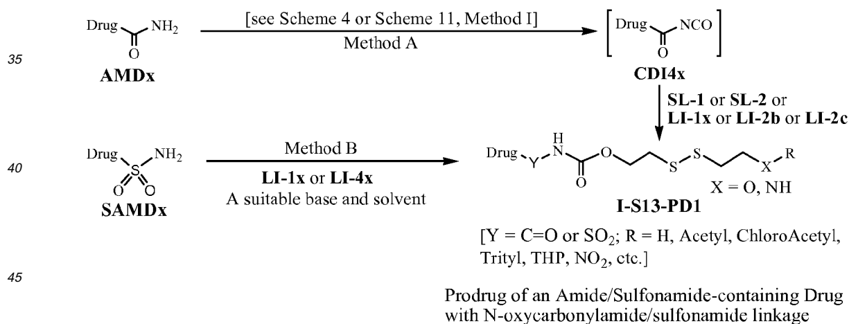
Scheme 13: Synthesis of Prodrugs of Amide/Sulfonamide-containing Drugs:
