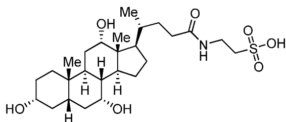
Taurocholic acid
