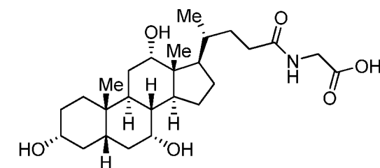
Glycocholic acid
