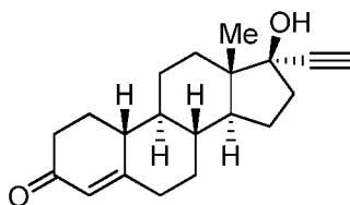
Norethindrone
