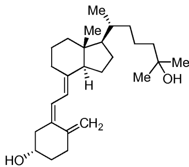
25-Hydroxyvitamin D 3
