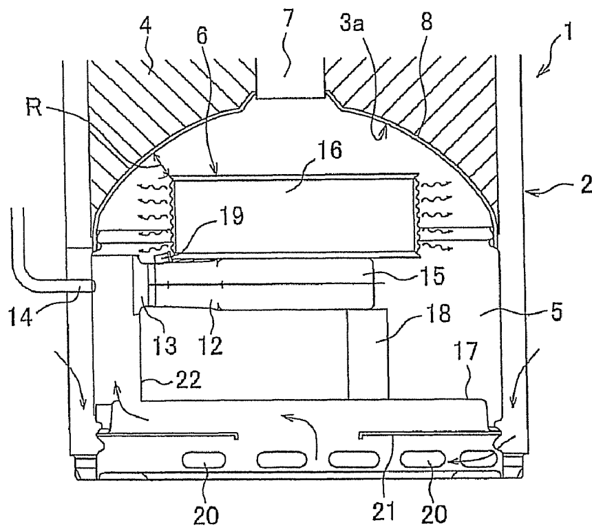
Fig. 4 PRIOR ART
