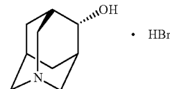
(3R,4S,5S,7S)-1-azaadamantan-4-ol hydrobromide
