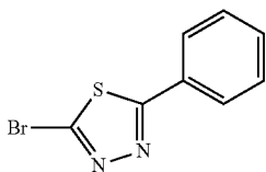
2-bromo-5-phenyl-1,3,4-thiadiazole
