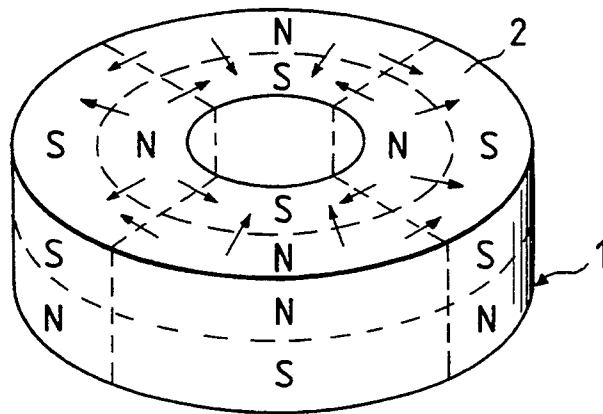
FIG. 4 PRIOR ART
