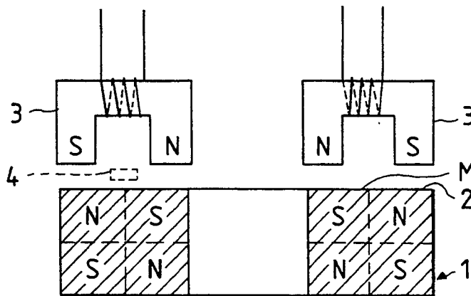
FIG. 5 PRIOR ART
