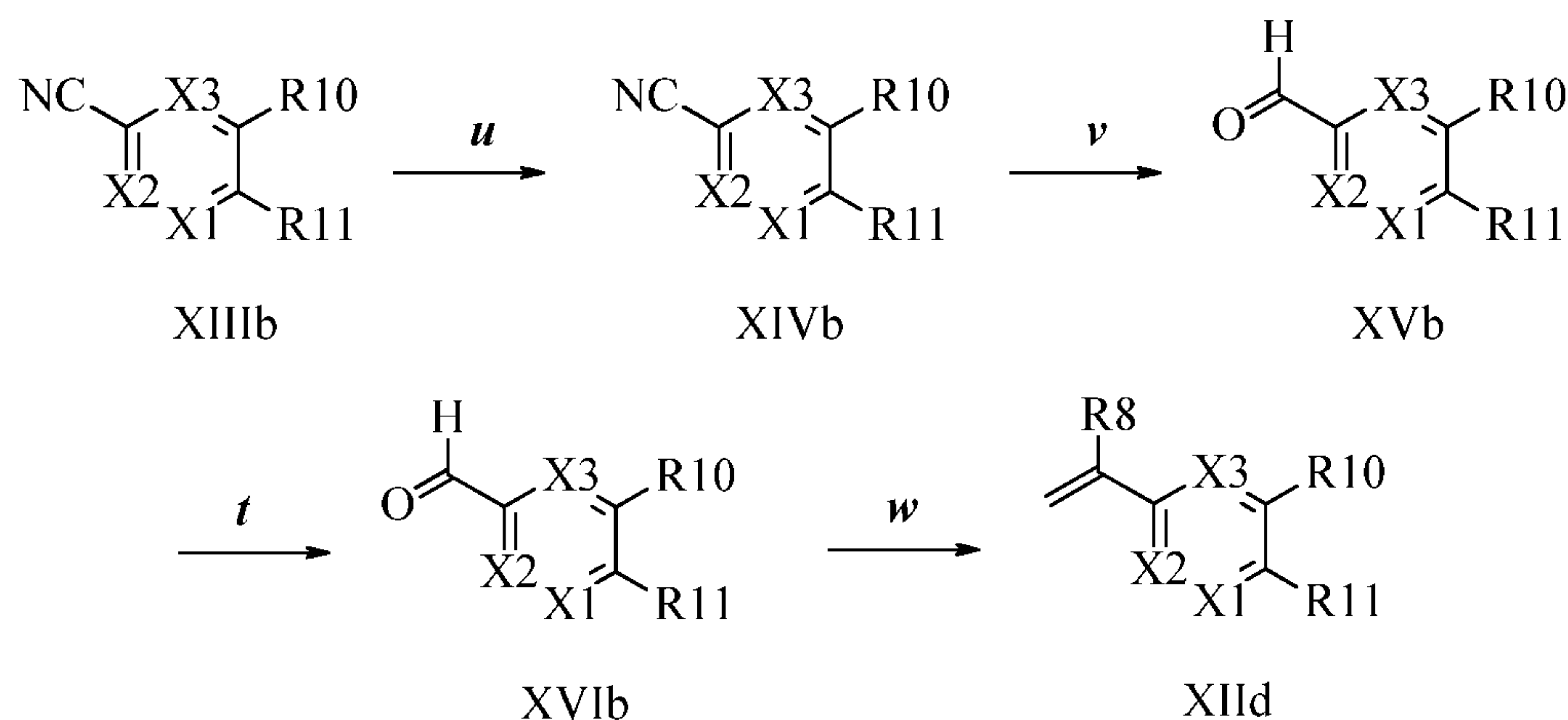
Scheme XVII
