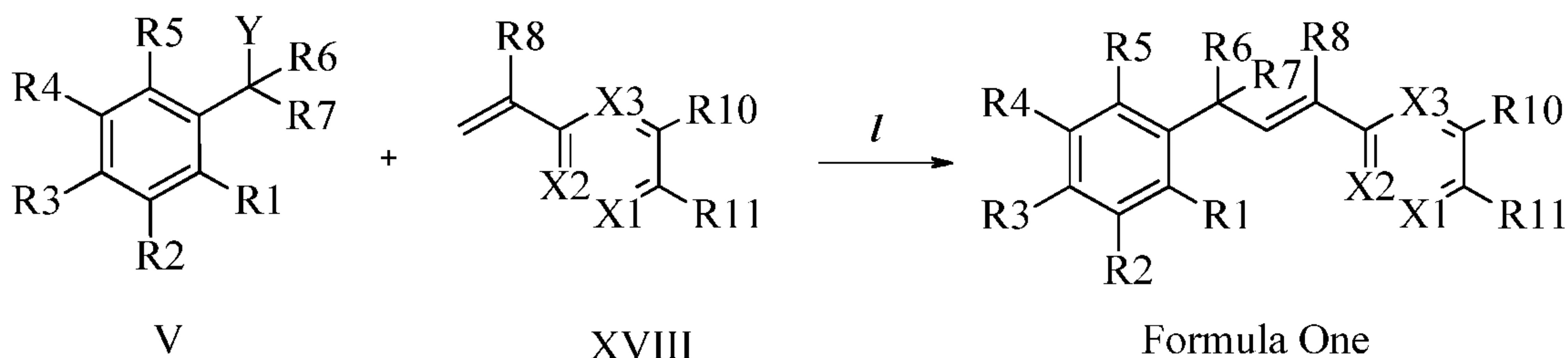
Scheme XXVI
