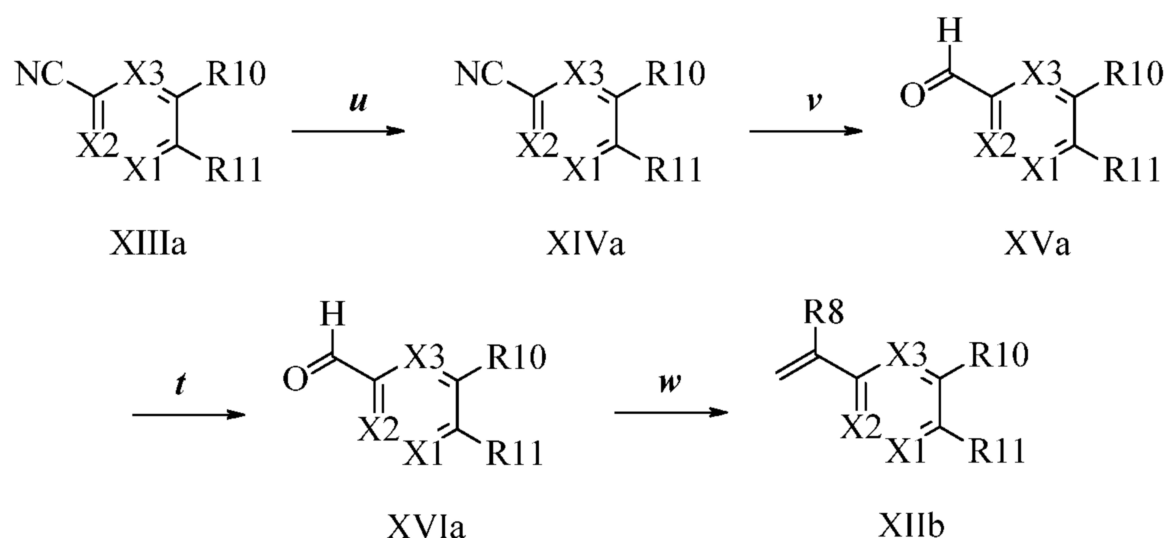
Scheme XIV
