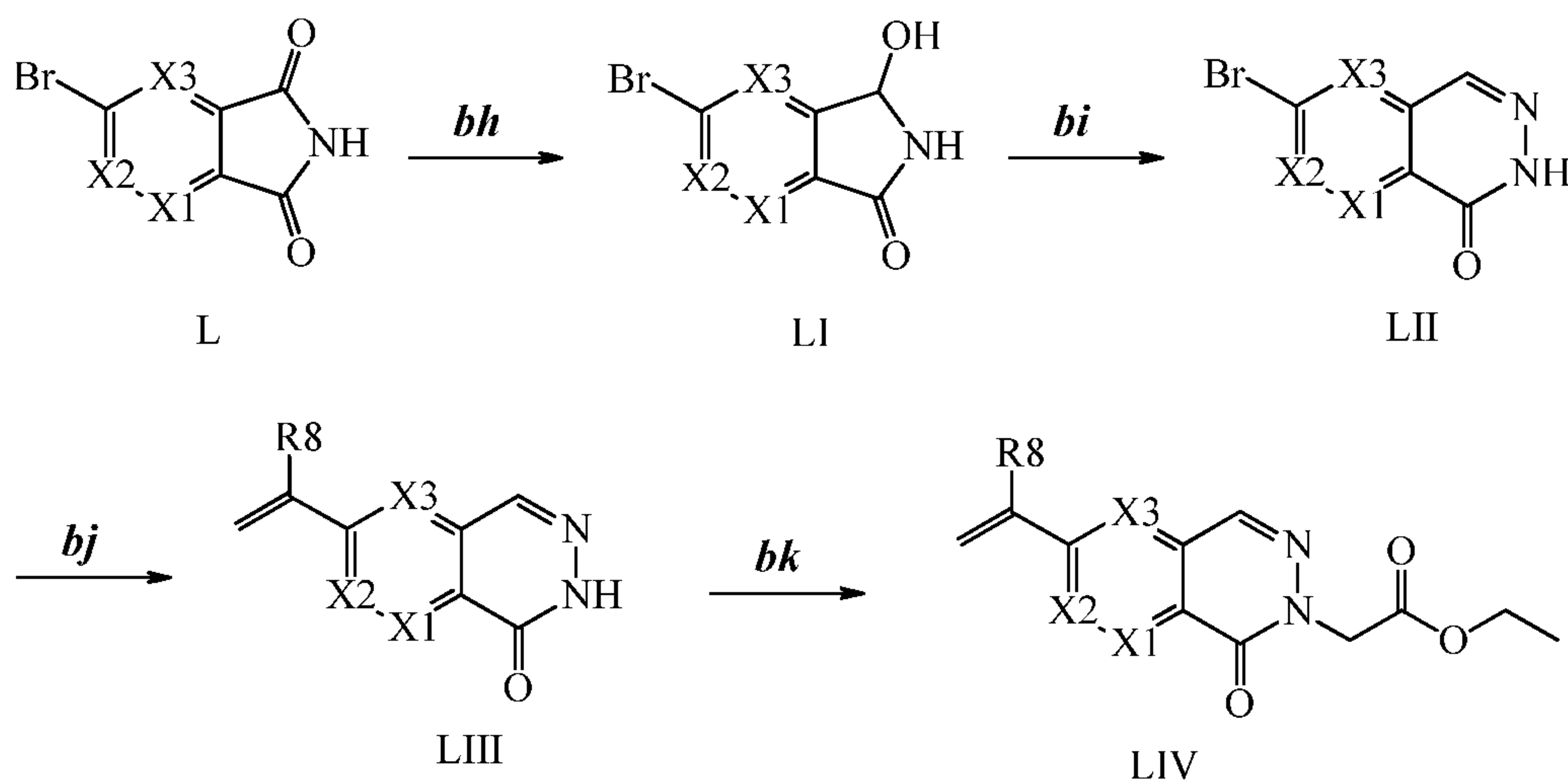
Scheme XXXVIII
