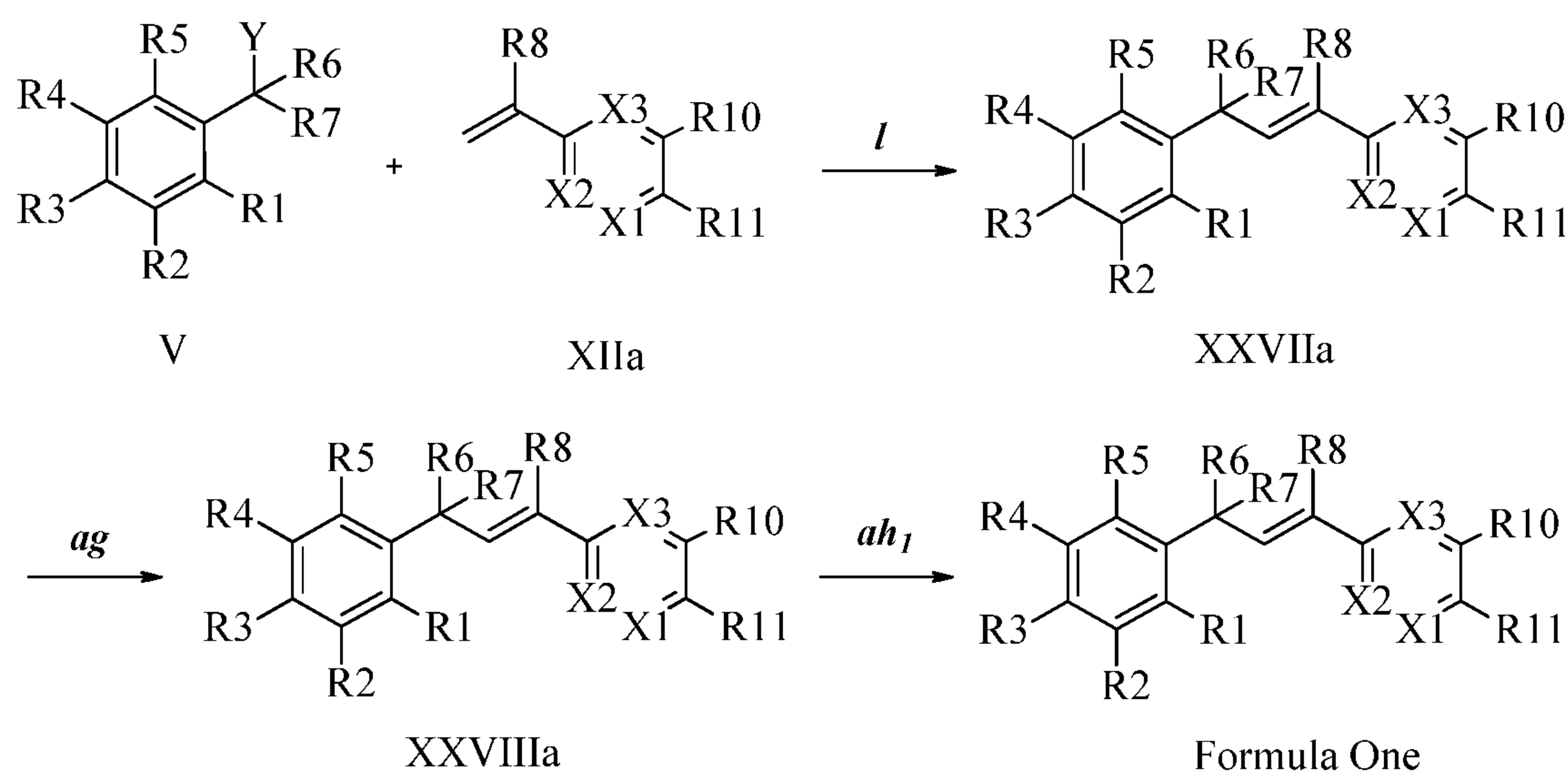
Scheme XX
