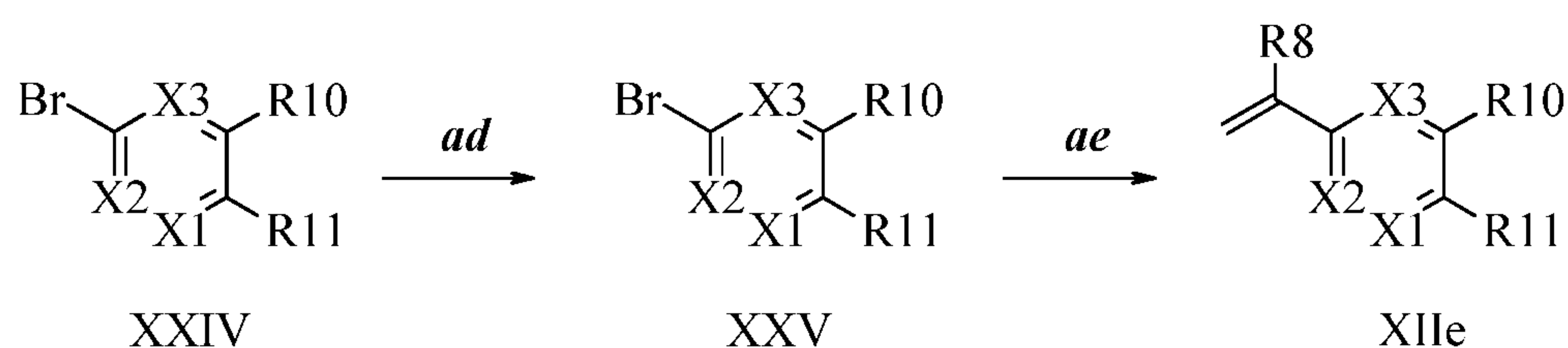
Scheme XVIII
