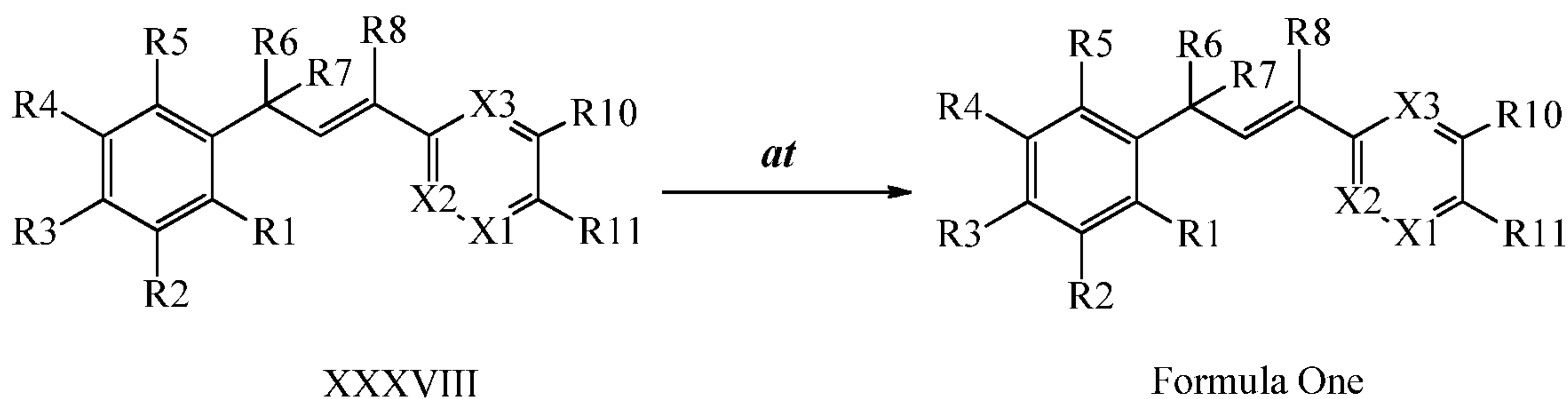
Scheme XXXII
