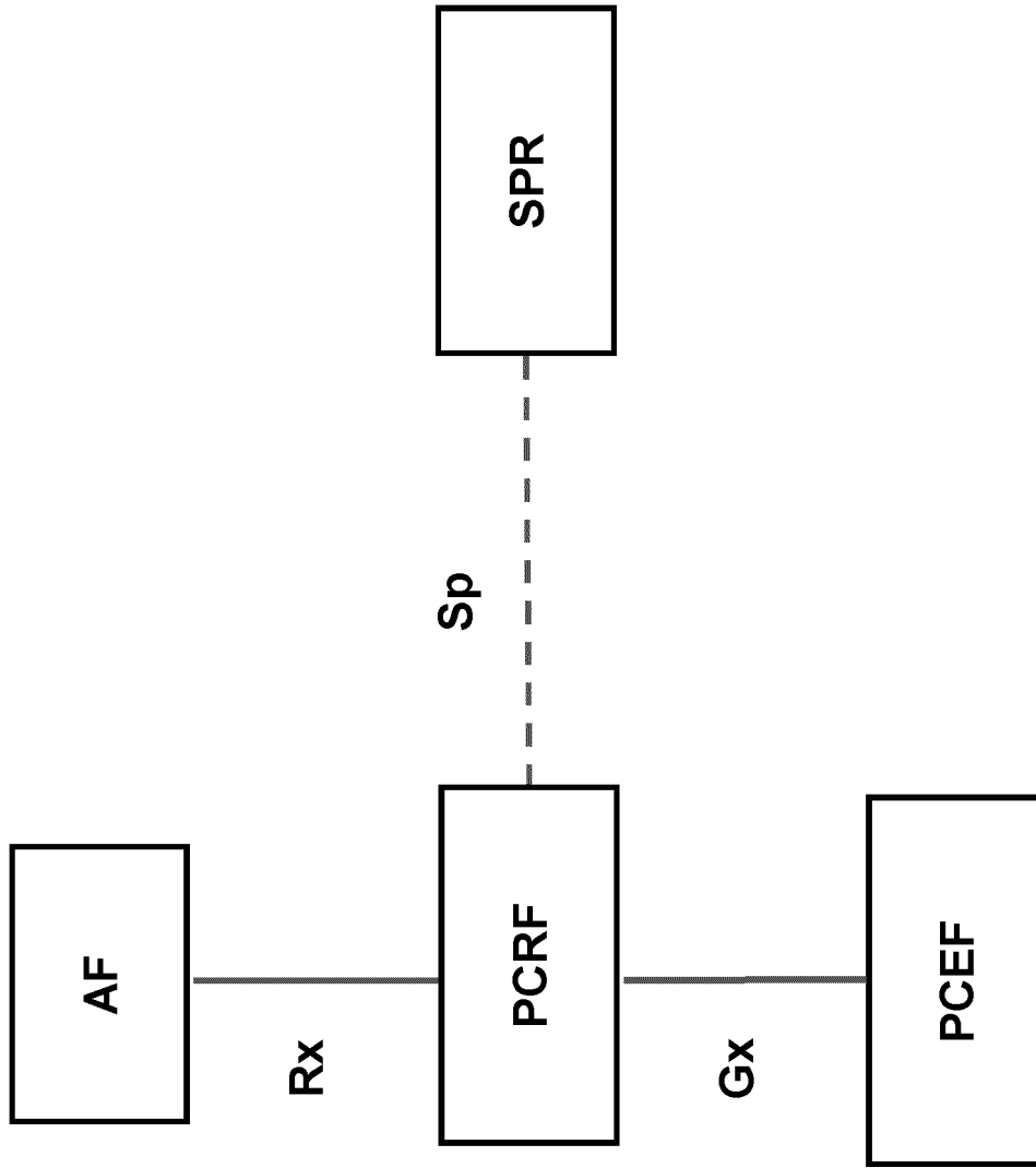
Fig. 1 3GPP Release-7 PCRF interfaces
