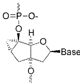
tricyclo-DNA
