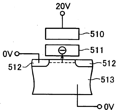
[During Write]
