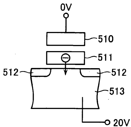
[During Erase]
