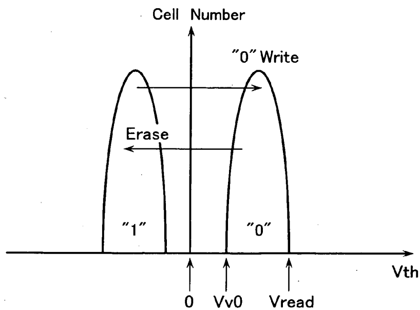
[Cell Array Threshold Voltage Distribution]
