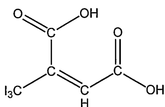
Citraconic Acid
