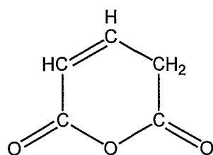
2-Pentendioic Anhydride
