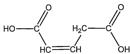
2-Pentendioic Acid
