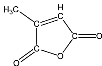
Citraconic Anhydride
