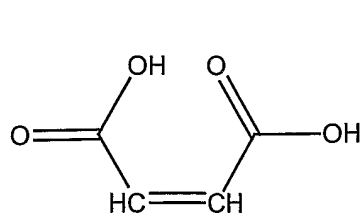
Maleic Acid
