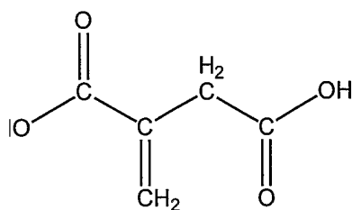
Itaconic Acid
