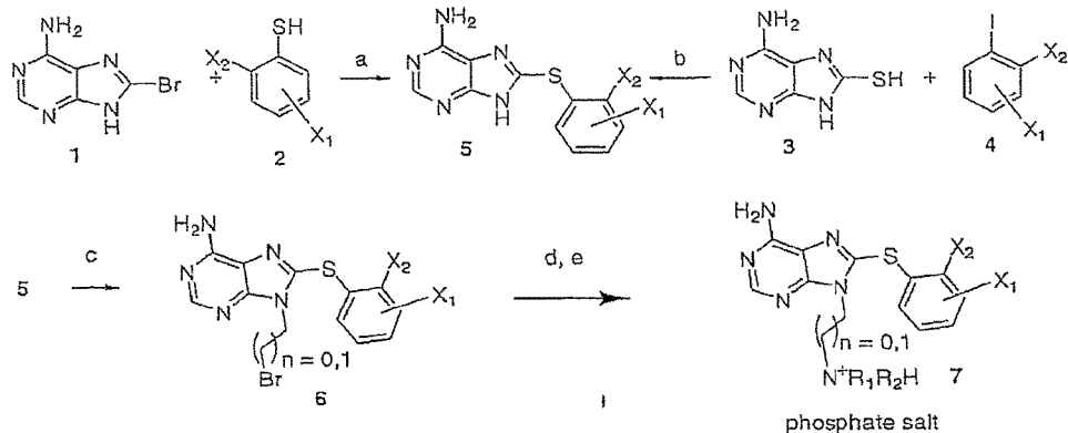
Scheme 1 a
