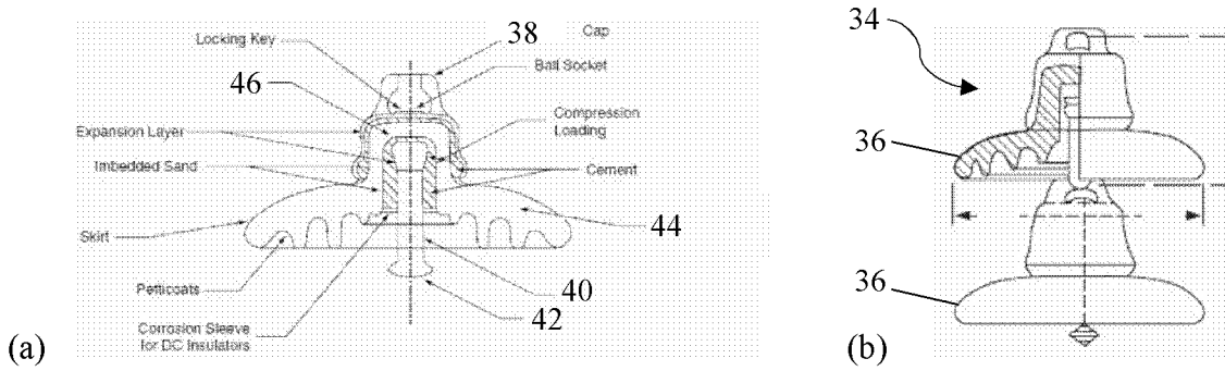
Fig.5 (Prior art)
