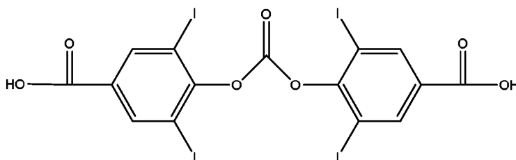
4,4'-(carbonylbis(oxy))bis(3,5-diiodobenzoic acid)
