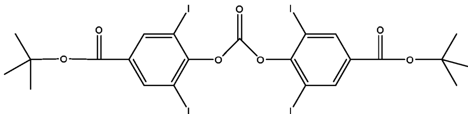
di-tert-butyl 4,4'-(carbonylbis(oxy))bis(3,5-diiodobenzoate)
