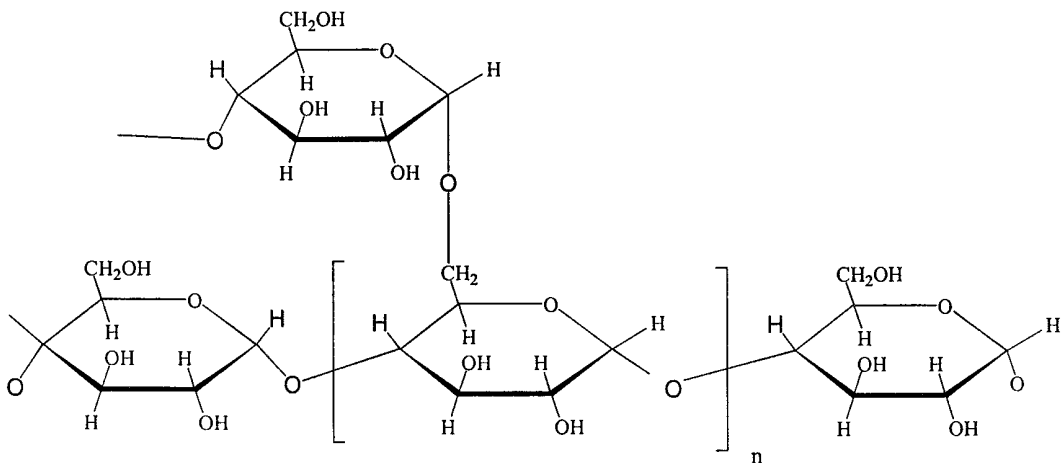
Starch - Amylopectin
