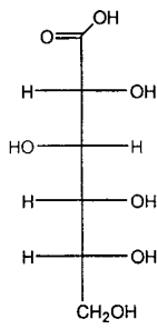
Gluconic Acid
