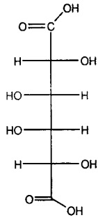
Mucic Acid
