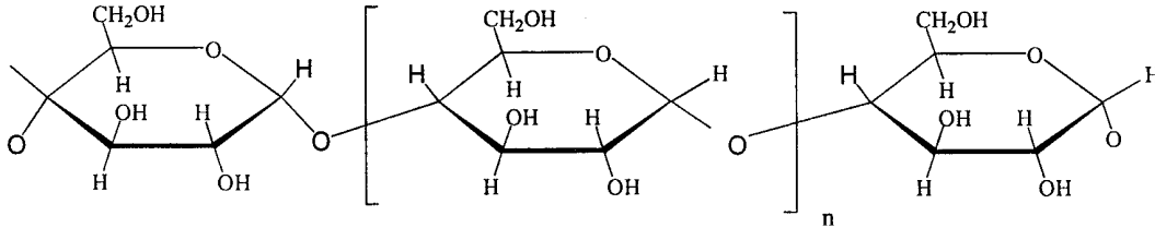
Starch - Amylose
