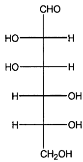
D-Mannose
